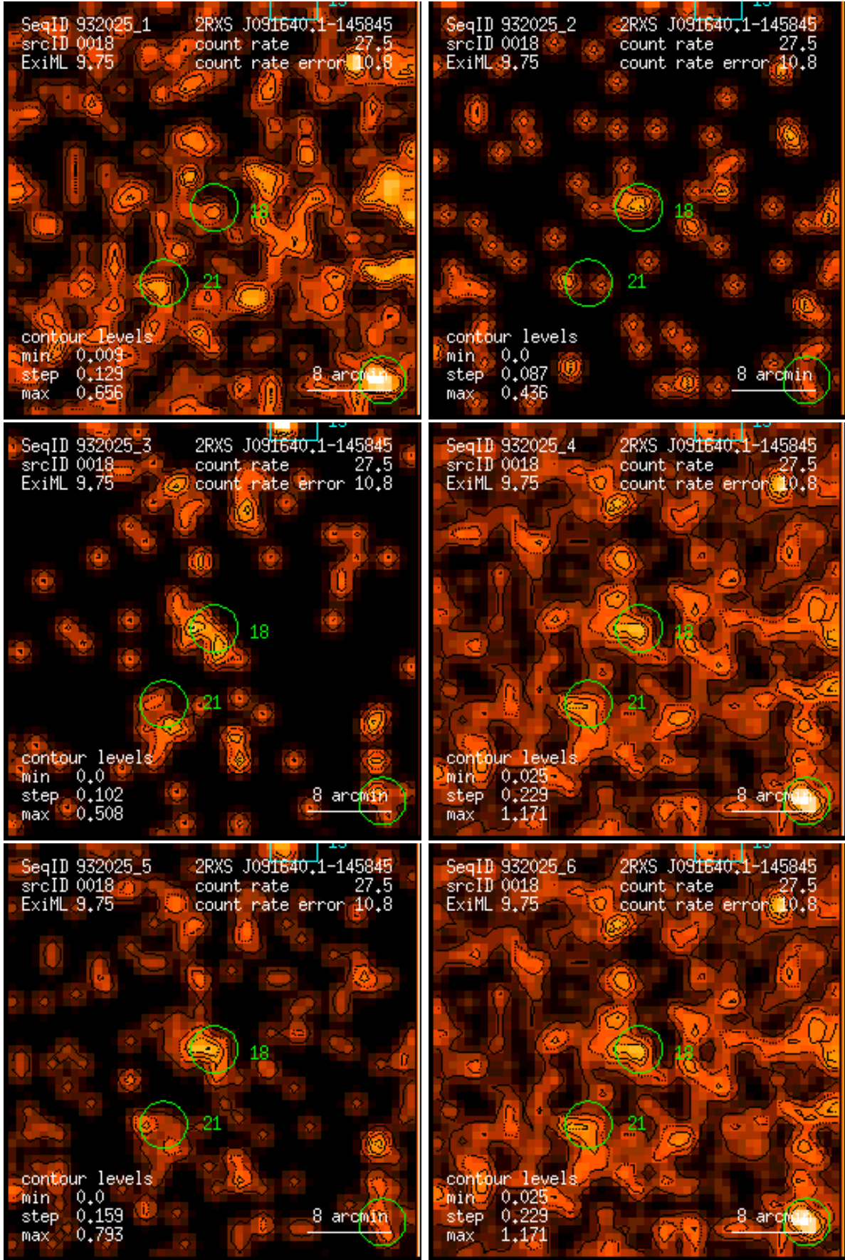
Figure 18: RASS 932025: detection 0018: band rate images, Gaussian filter: (1) PSPC channels 11 – 41, (2) 52 – 90, (3) 91 – 201, (4) 11 – 235, (5) 52 – 201, (6) 11 – 201. Broad band rates in counts/ks. Band rate contour levels in counts/ks/arcmin 2 .
