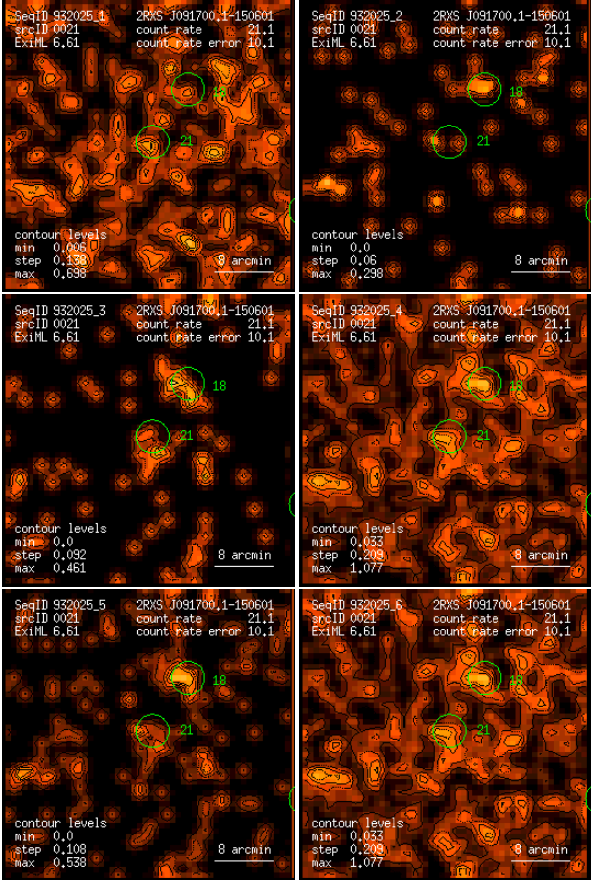
Figure 21: RASS 932025: detection 0021: band rate images, Gaussian filter: (1) PSPC channels 11 – 41, (2) 52 – 90, (3) 91 – 201, (4) 11 – 235, (5) 52 – 201, (6) 11 – 201. Broad band rates in counts/ks. Band rate contour levels in counts/ks/arcmin 2 .
