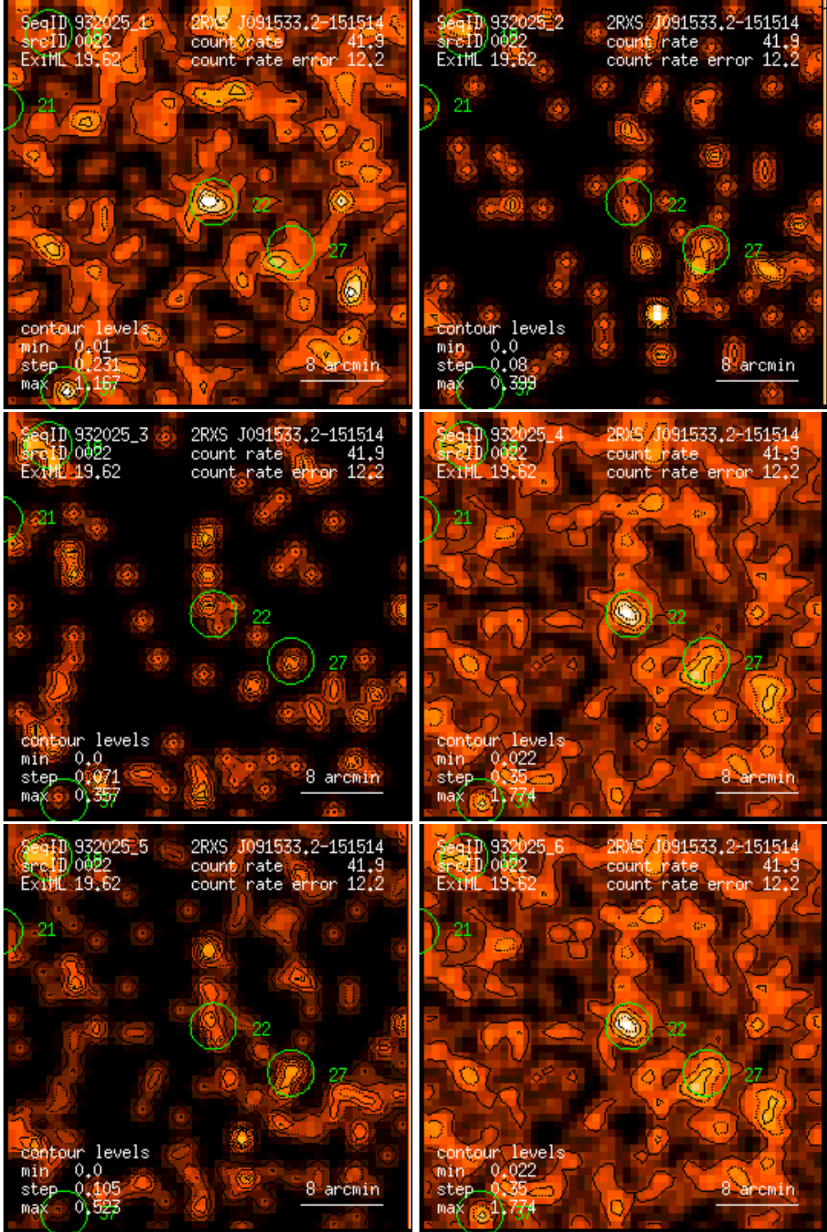
Figure 22: RASS 932025: detection 0022: band rate images, Gaussian filter: (1) PSPC channels 11 – 41, (2) 52 – 90, (3) 91 – 201, (4) 11 – 235, (5) 52 – 201, (6) 11 – 201. Broad band rates in counts/ks. Band rate contour levels in counts/ks/arcmin 2 .
