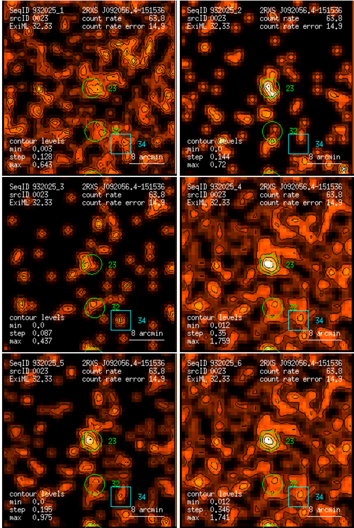
Figure 23: RASS 932025: detection 0023: band rate images, Gaussian filter: (1) PSPC channels 11 – 41, (2) 52 – 90, (3) 91 – 201, (4) 11 – 235, (5) 52 – 201, (6) 11 – 201. Broad band rates in counts/ks. Band rate contour levels in counts/ks/arcmin 2 .
