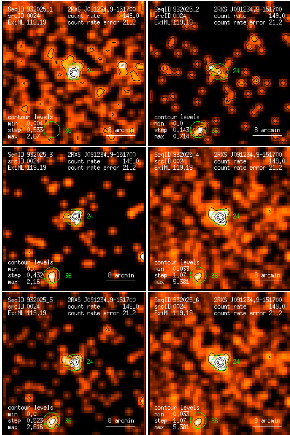
Figure 24: RASS 932025: detection 0024: band rate images, Gaussian filter: (1) PSPC channels 11 – 41, (2) 52 – 90, (3) 91 – 201, (4) 11 – 235, (5) 52 – 201, (6) 11 – 201. Broad band rates in counts/ks. Band rate contour levels in counts/ks/arcmin 2 .
