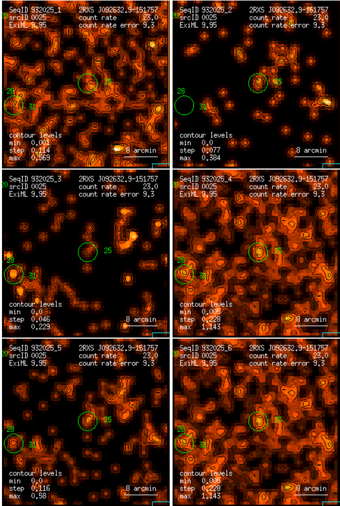
Figure 25: RASS 932025: detection 0025: band rate images, Gaussian filter: (1) PSPC channels 11 – 41, (2) 52 – 90, (3) 91 – 201, (4) 11 – 235, (5) 52 – 201, (6) 11 – 201. Broad band rates in counts/ks. Band rate contour levels in counts/ks/arcmin 2 .
