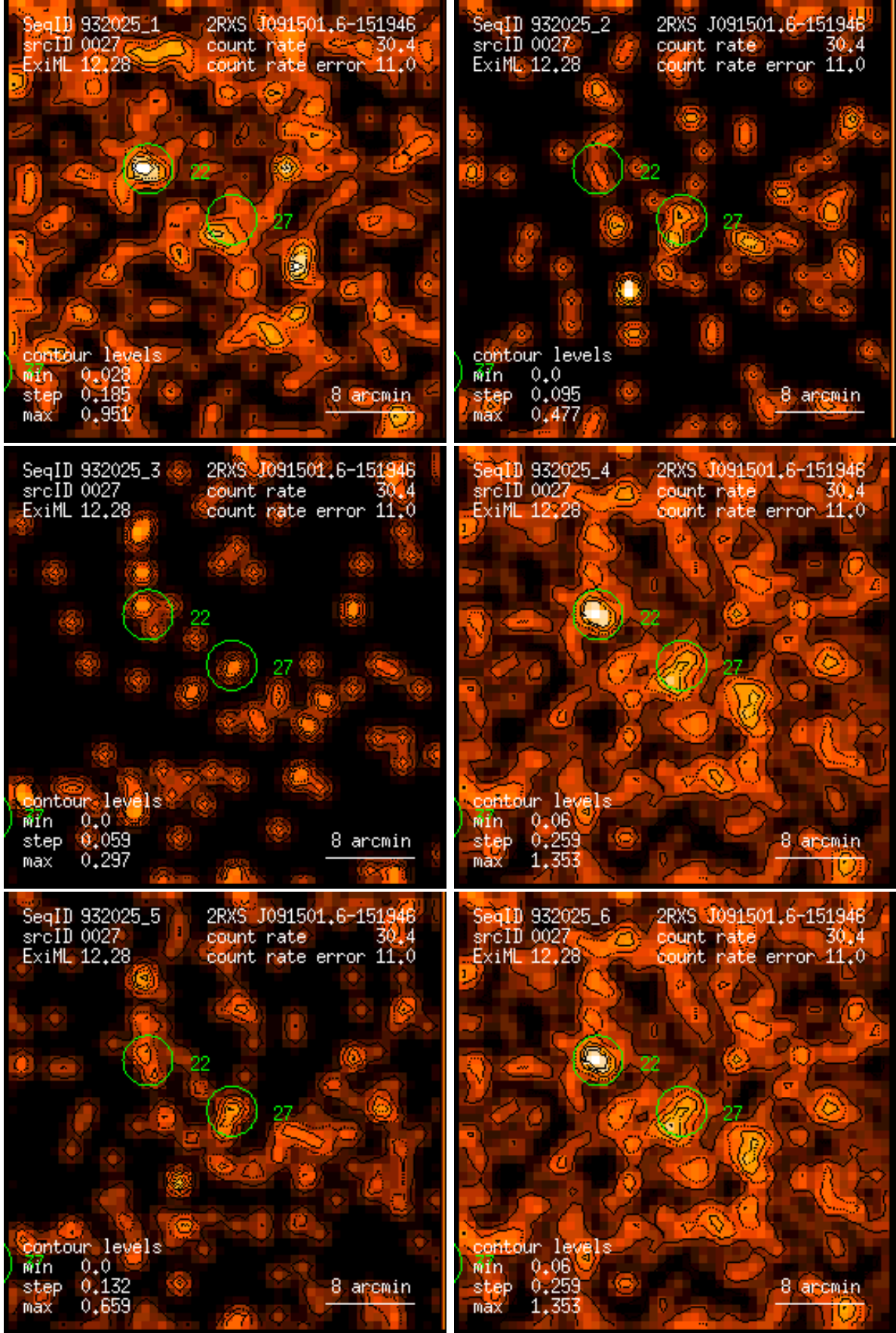
Figure 27: RASS 932025: detection 0027: band rate images, Gaussian filter: (1) PSPC channels 11 – 41, (2) 52 – 90, (3) 91 – 201, (4) 11 – 235, (5) 52 – 201, (6) 11 – 201. Broad band rates in counts/ks. Band rate contour levels in counts/ks/arcmin 2 .
