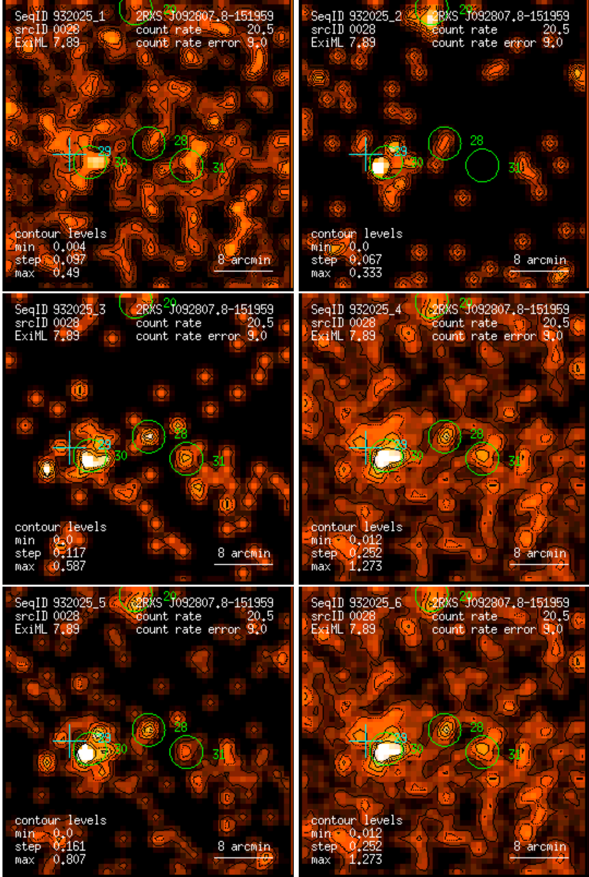
Figure 28: RASS 932025: detection 0028: band rate images, Gaussian filter: (1) PSPC channels 11 – 41, (2) 52 – 90, (3) 91 – 201, (4) 11 – 235, (5) 52 – 201, (6) 11 – 201. Broad band rates in counts/ks. Band rate contour levels in counts/ks/arcmin 2 .
