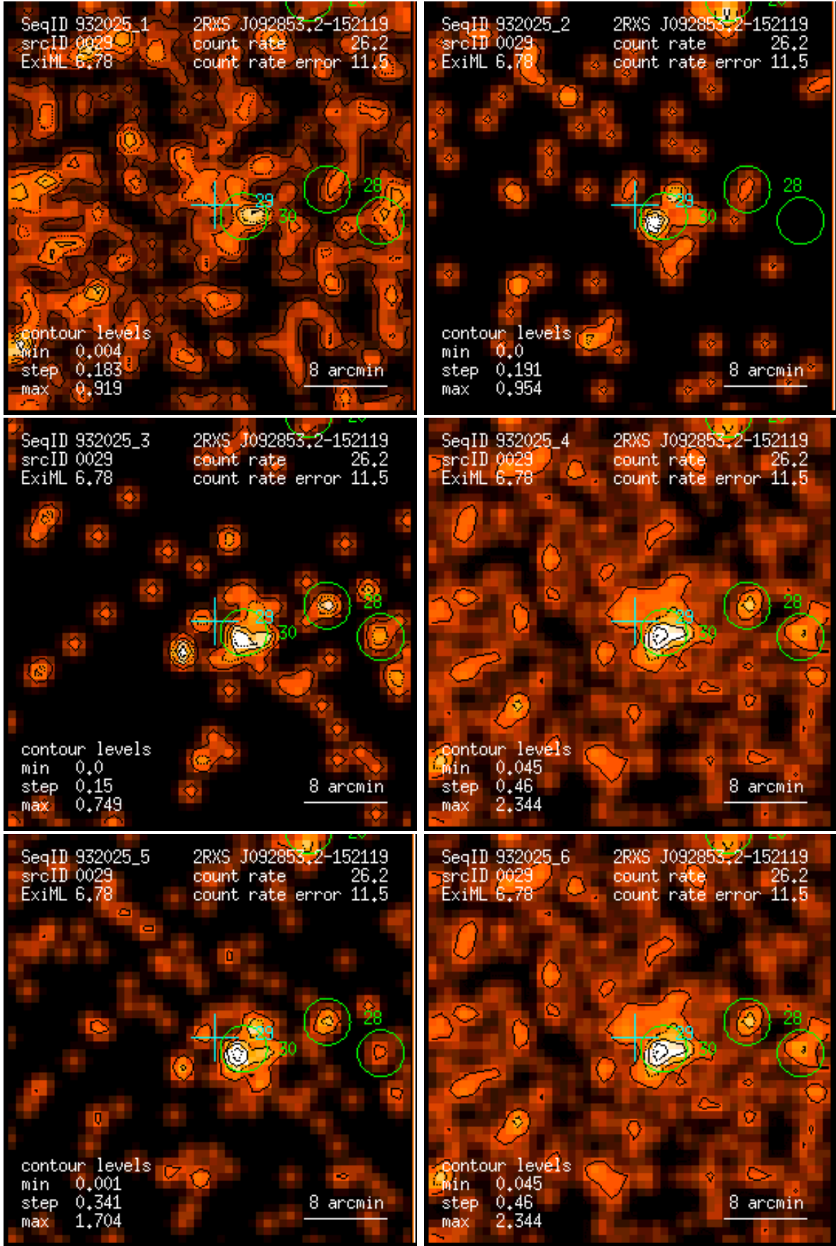
Figure 29: RASS 932025: detection 0029: band rate images, Gaussian filter: (1) PSPC channels 11 – 41, (2) 52 – 90, (3) 91 – 201, (4) 11 – 235, (5) 52 – 201, (6) 11 – 201. Broad band rates in counts/ks. Band rate contour levels in counts/ks/arcmin 2 .
