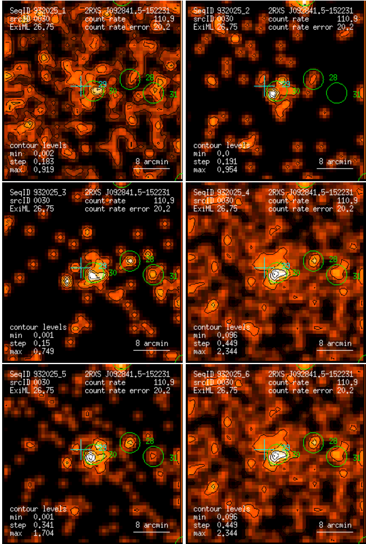
Figure 30: RASS 932025: detection 0030: band rate images, Gaussian filter: (1) PSPC channels 11 – 41, (2) 52 – 90, (3) 91 – 201, (4) 11 – 235, (5) 52 – 201, (6) 11 – 201. Broad band rates in counts/ks. Band rate contour levels in counts/ks/arcmin 2 .
