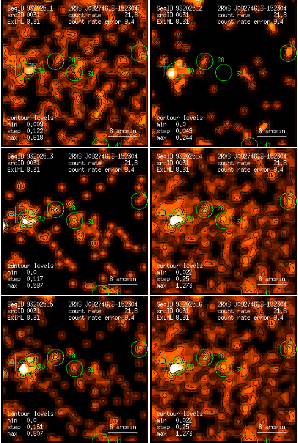
Figure 31: RASS 932025: detection 0031: band rate images, Gaussian filter: (1) PSPC channels 11 – 41, (2) 52 – 90, (3) 91 – 201, (4) 11 – 235, (5) 52 – 201, (6) 11 – 201. Broad band rates in counts/ks. Band rate contour levels in counts/ks/arcmin 2 .
