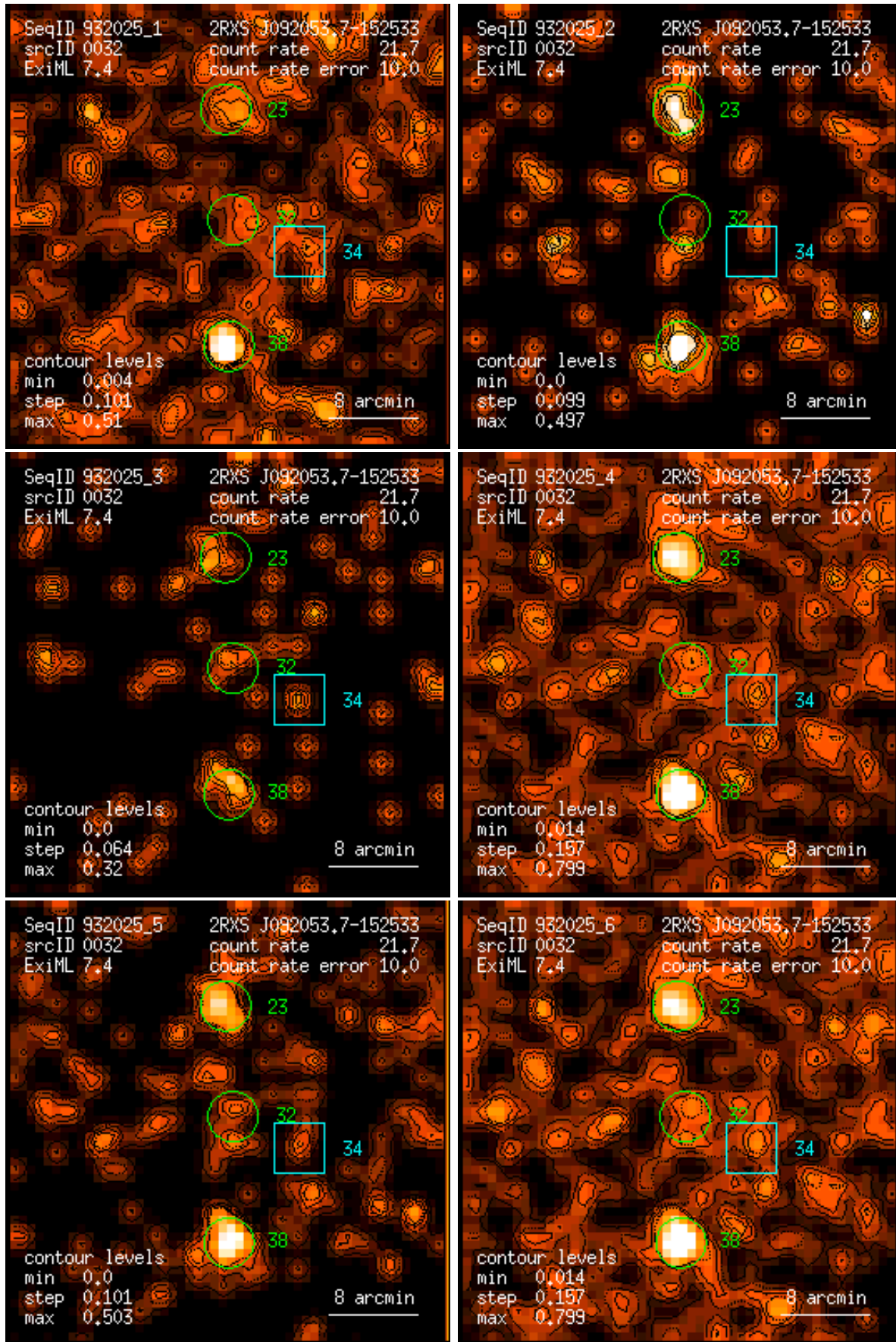
Figure 32: RASS 932025: detection 0032: band rate images, Gaussian filter: (1) PSPC channels 11 – 41, (2) 52 – 90, (3) 91 – 201, (4) 11 – 235, (5) 52 – 201, (6) 11 – 201. Broad band rates in counts/ks. Band rate contour levels in counts/ks/arcmin 2 .
