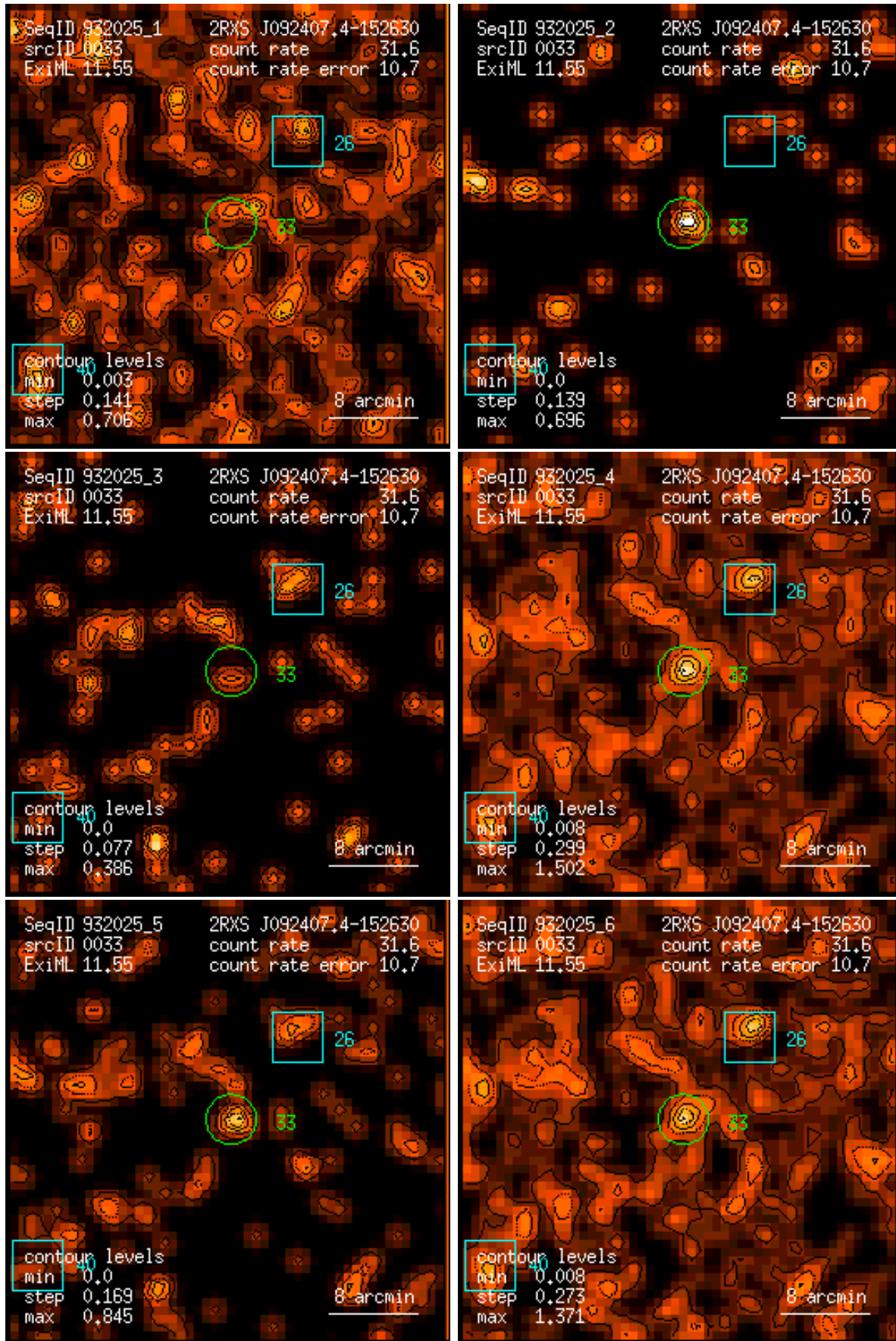
Figure 33: RASS 932025: detection 0033: band rate images, Gaussian filter: (1) PSPC channels 11 – 41, (2) 52 – 90, (3) 91 – 201, (4) 11 – 235, (5) 52 – 201, (6) 11 – 201. Broad band rates in counts/ks. Band rate contour levels in counts/ks/arcmin 2 .
