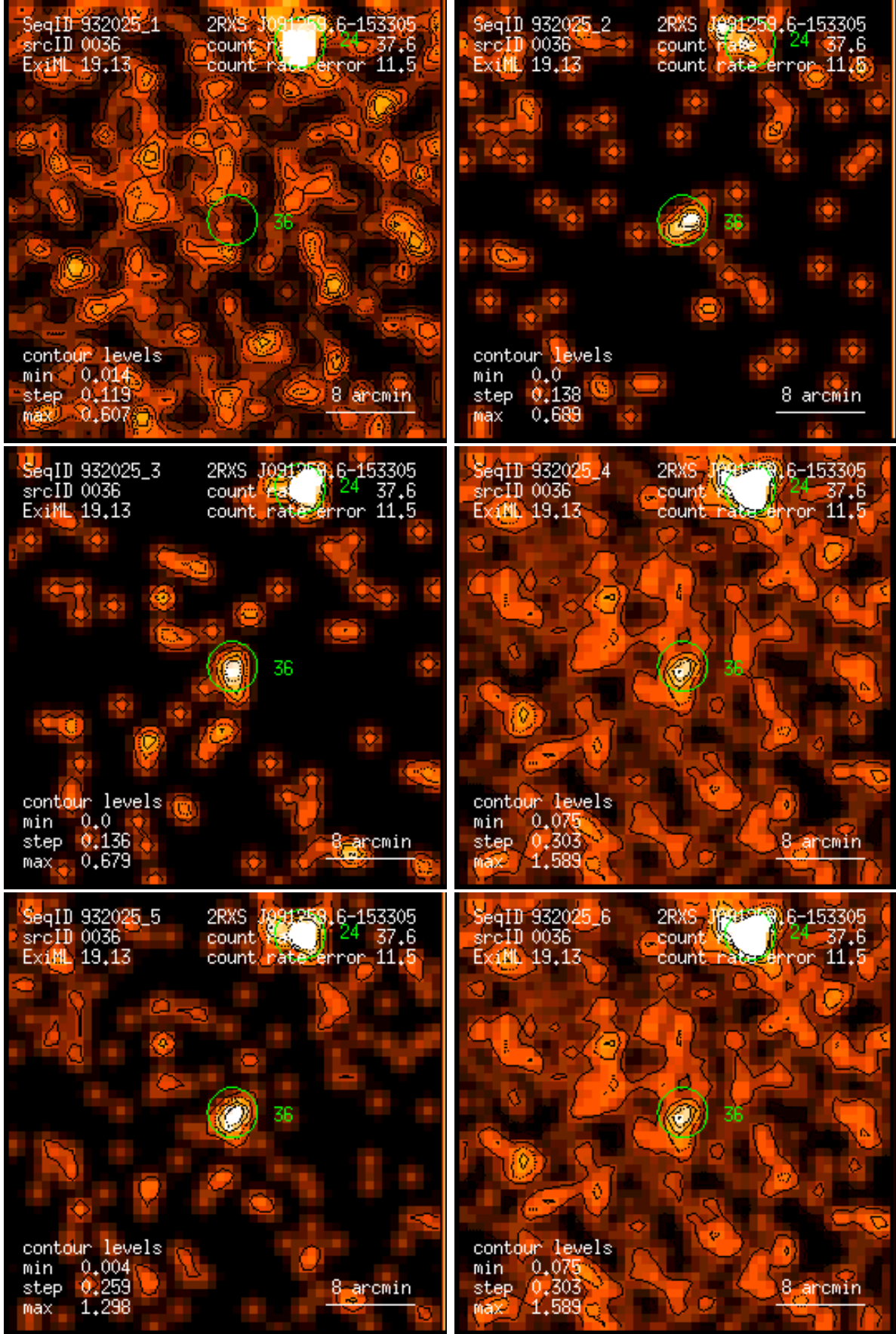
Figure 36: RASS 932025: detection 0036: band rate images, Gaussian filter: (1) PSPC channels 11 – 41, (2) 52 – 90, (3) 91 – 201, (4) 11 – 235, (5) 52 – 201, (6) 11 – 201. Broad band rates in counts/ks. Band rate contour levels in counts/ks/arcmin 2 .
