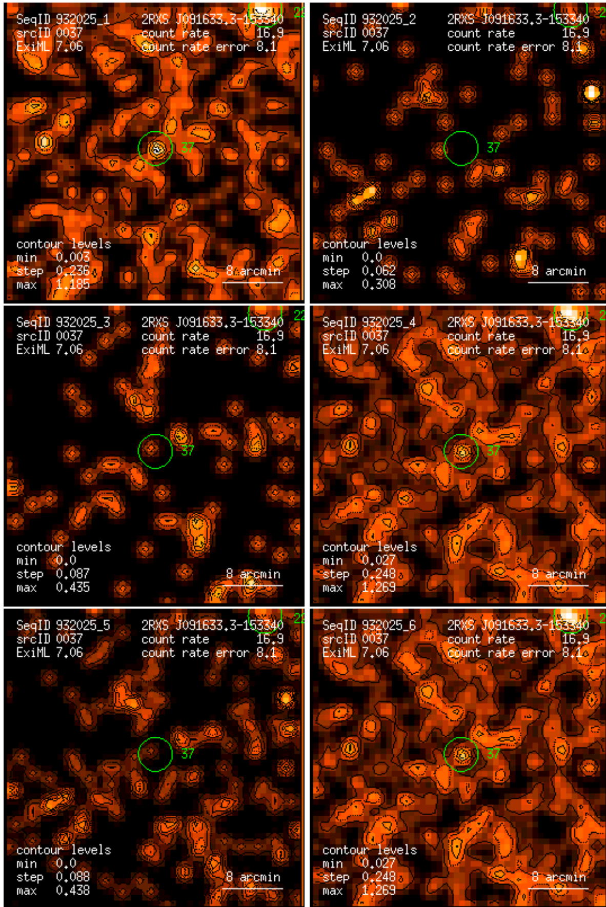
Figure 37: RASS 932025: detection 0037: band rate images, Gaussian filter: (1) PSPC channels 11 – 41, (2) 52 – 90, (3) 91 – 201, (4) 11 – 235, (5) 52 – 201, (6) 11 – 201. Broad band rates in counts/ks. Band rate contour levels in counts/ks/arcmin 2 .
