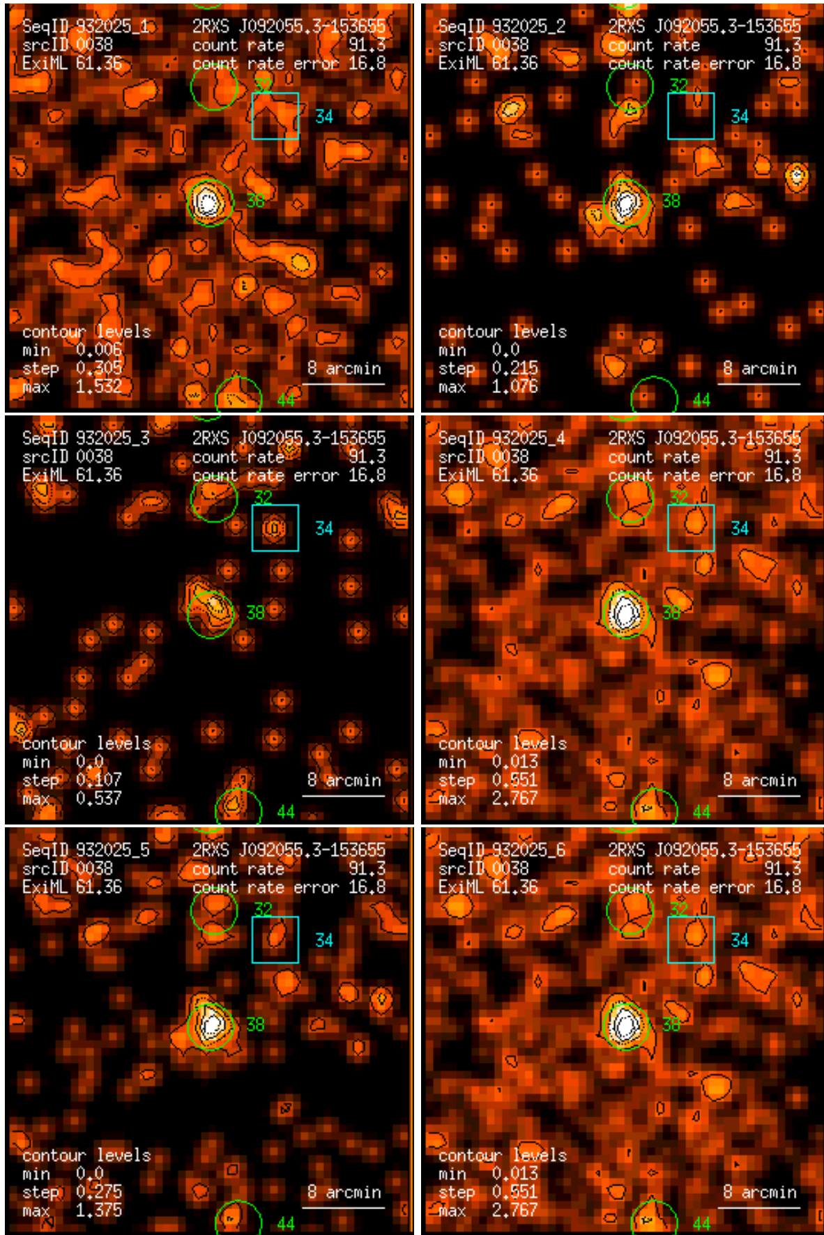
Figure 38: RASS 932025: detection 0038: band rate images, Gaussian filter: (1) PSPC channels 11 – 41, (2) 52 – 90, (3) 91 – 201, (4) 11 – 235, (5) 52 – 201, (6) 11 – 201. Broad band rates in counts/ks. Band rate contour levels in counts/ks/arcmin 2 .
