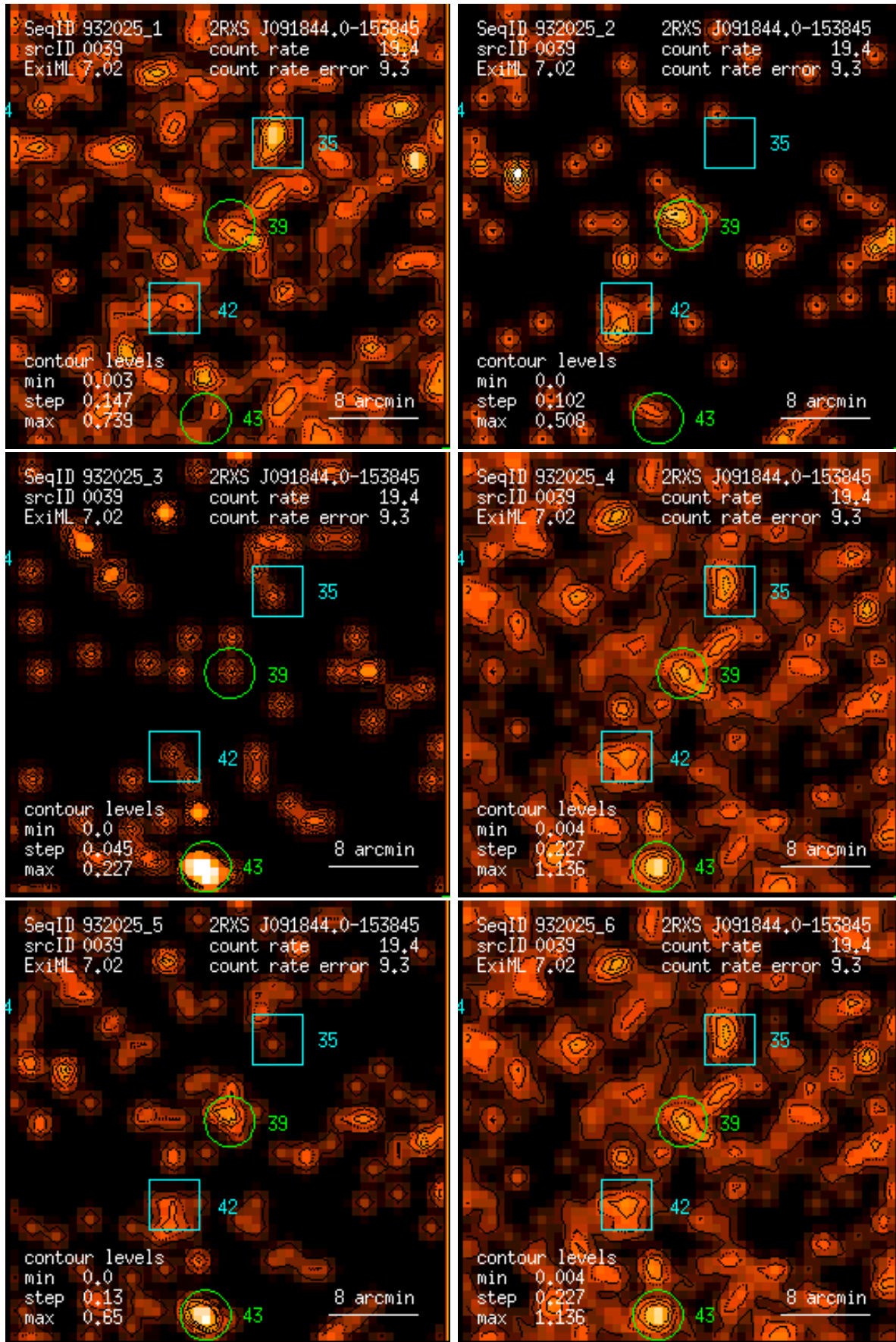
Figure 39: RASS 932025: detection 0039: band rate images, Gaussian filter: (1) PSPC channels 11 – 41, (2) 52 – 90, (3) 91 – 201, (4) 11 – 235, (5) 52 – 201, (6) 11 – 201. Broad band rates in counts/ks. Band rate contour levels in counts/ks/arcmin 2 .
