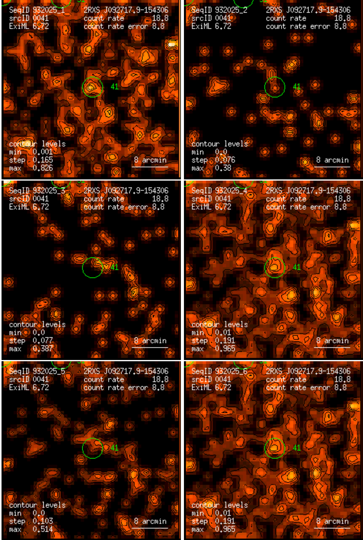
Figure 41: RASS 932025: detection 0041: band rate images, Gaussian filter: (1) PSPC channels 11 – 41, (2) 52 – 90, (3) 91 – 201, (4) 11 – 235, (5) 52 – 201, (6) 11 – 201. Broad band rates in counts/ks. Band rate contour levels in counts/ks/arcmin 2 .
