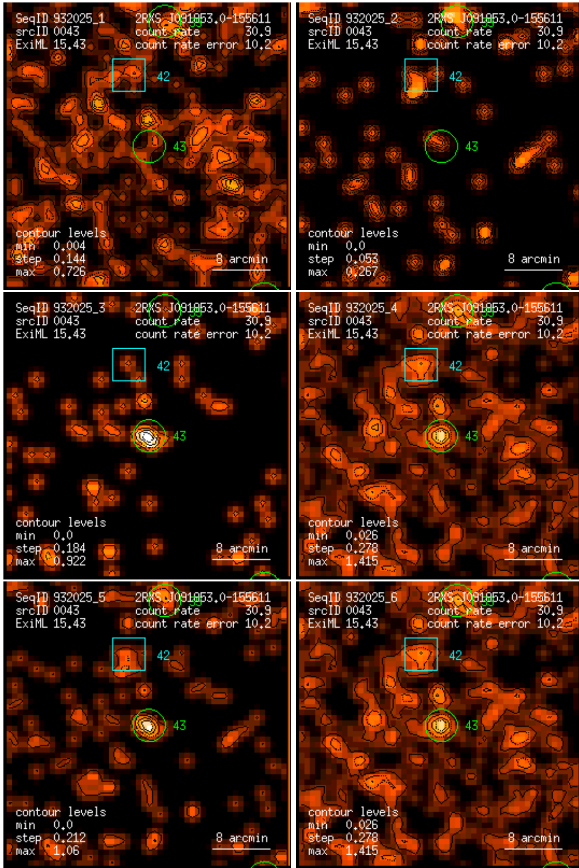
Figure 43: RASS 932025: detection 0043: band rate images, Gaussian filter: (1) PSPC channels 11 – 41, (2) 52 – 90, (3) 91 – 201, (4) 11 – 235, (5) 52 – 201, (6) 11 – 201. Broad band rates in counts/ks. Band rate contour levels in counts/ks/arcmin 2 .
