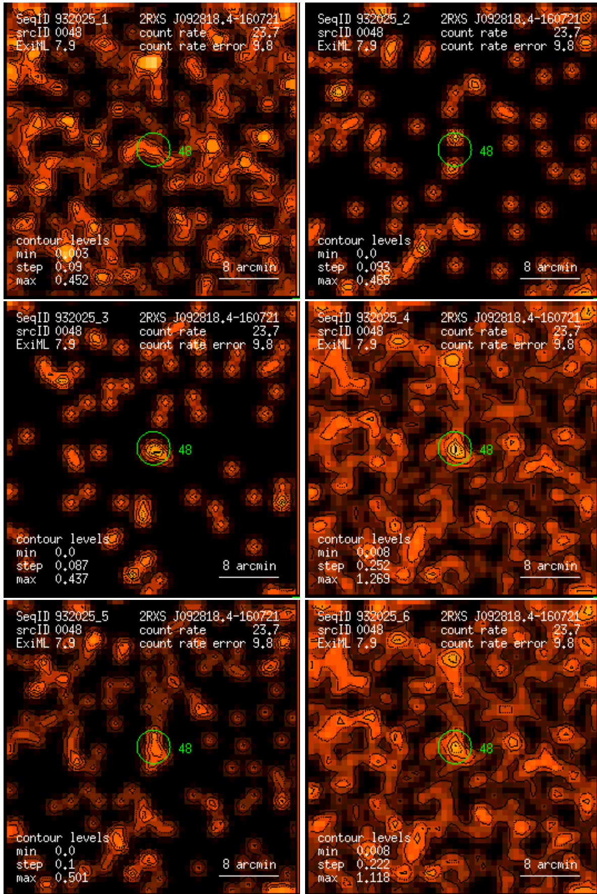
Figure 48: RASS 932025: detection 0048: band rate images, Gaussian filter: (1) PSPC channels 11 – 41, (2) 52 – 90, (3) 91 – 201, (4) 11 – 235, (5) 52 – 201, (6) 11 – 201. Broad band rates in counts/ks. Band rate contour levels in counts/ks/arcmin 2 .
