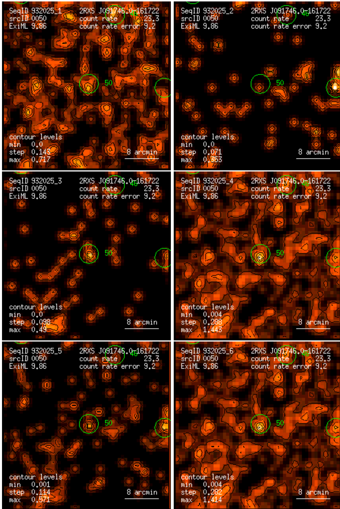
Figure 50: RASS 932025: detection 0050: band rate images, Gaussian filter: (1) PSPC channels 11 – 41, (2) 52 – 90, (3) 91 – 201, (4) 11 – 235, (5) 52 – 201, (6) 11 – 201. Broad band rates in counts/ks. Band rate contour levels in counts/ks/arcmin 2 .
