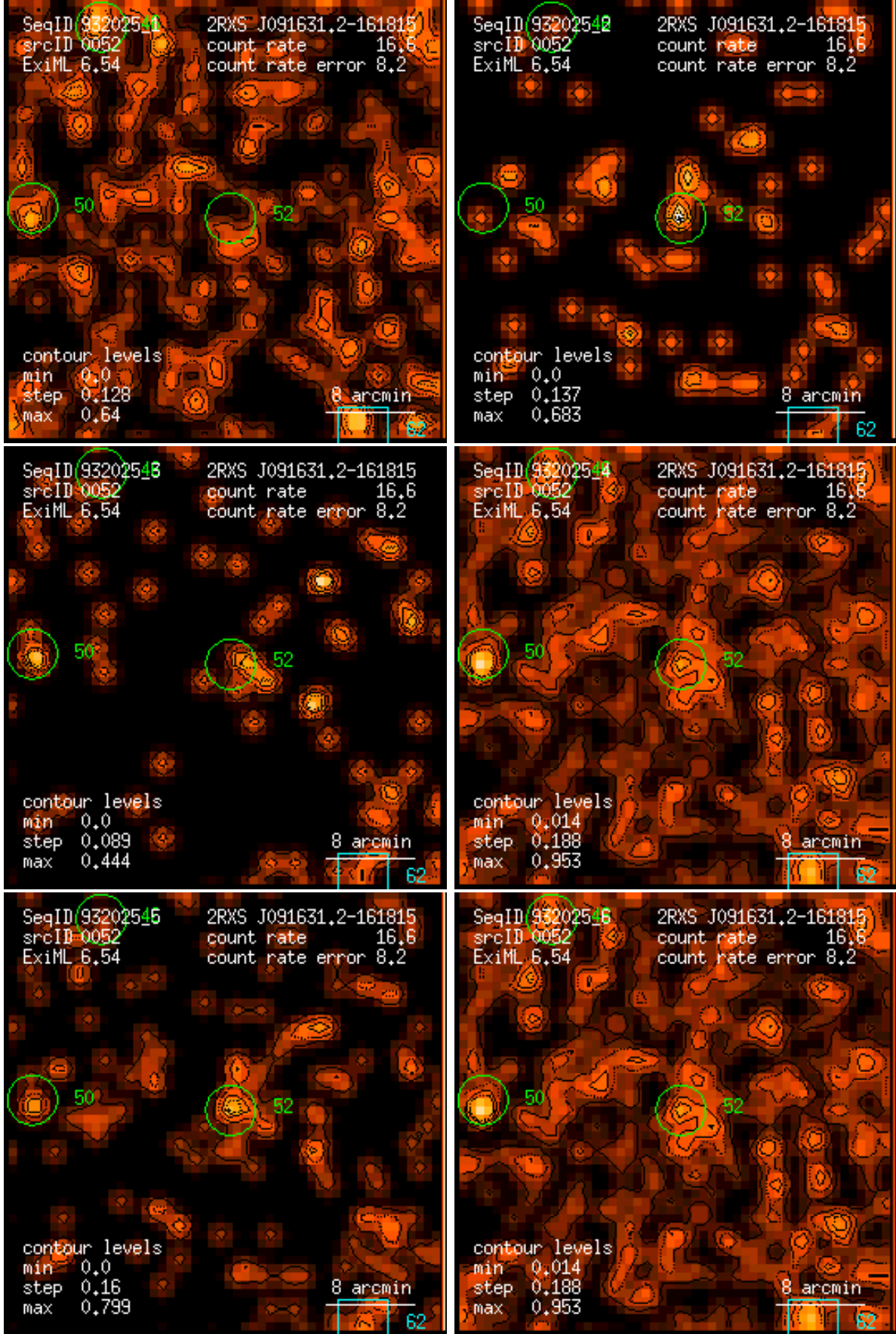
Figure 52: RASS 932025: detection 0052: band rate images, Gaussian filter: (1) PSPC channels 11 – 41, (2) 52 – 90, (3) 91 – 201, (4) 11 – 235, (5) 52 – 201, (6) 11 – 201. Broad band rates in counts/ks. Band rate contour levels in counts/ks/arcmin 2 .
