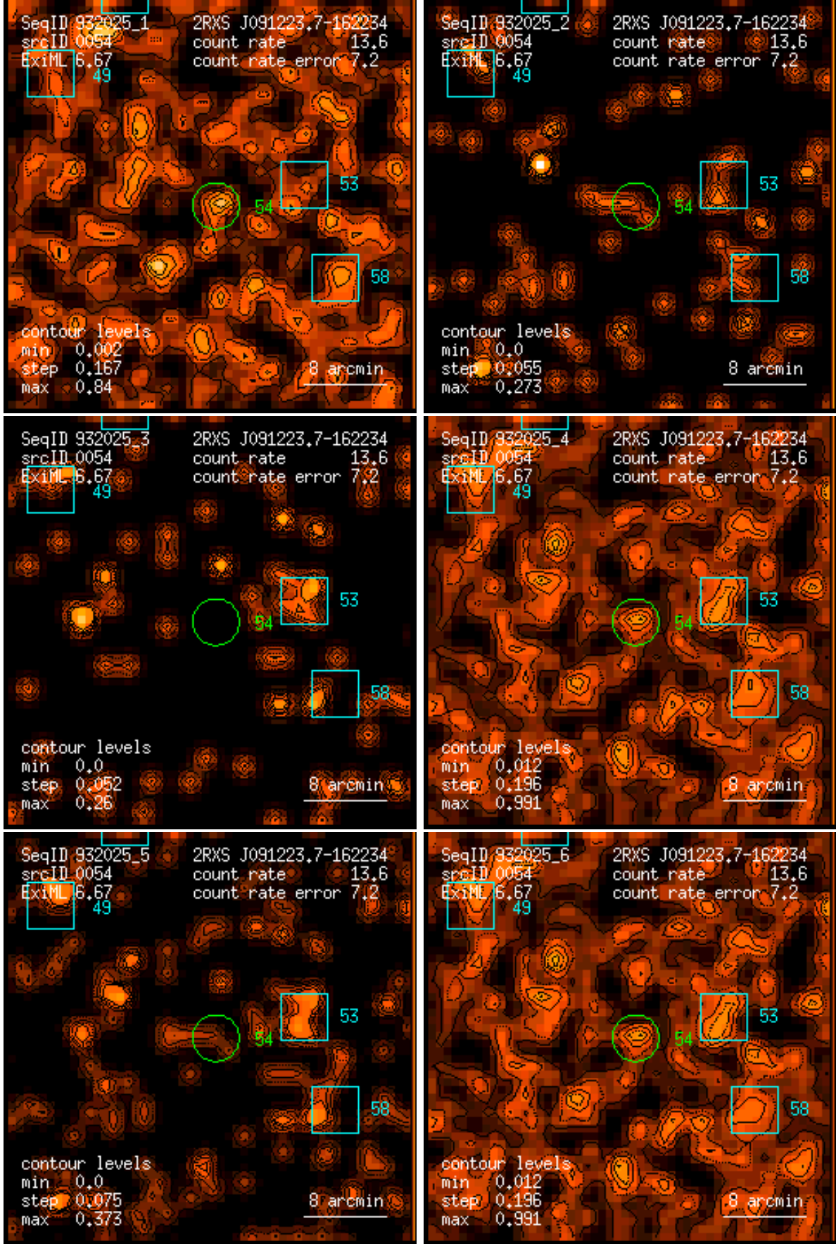
Figure 54: RASS 932025: detection 0054: band rate images, Gaussian filter: (1) PSPC channels 11 – 41, (2) 52 – 90, (3) 91 – 201, (4) 11 – 235, (5) 52 – 201, (6) 11 – 201. Broad band rates in counts/ks. Band rate contour levels in counts/ks/arcmin 2 .
