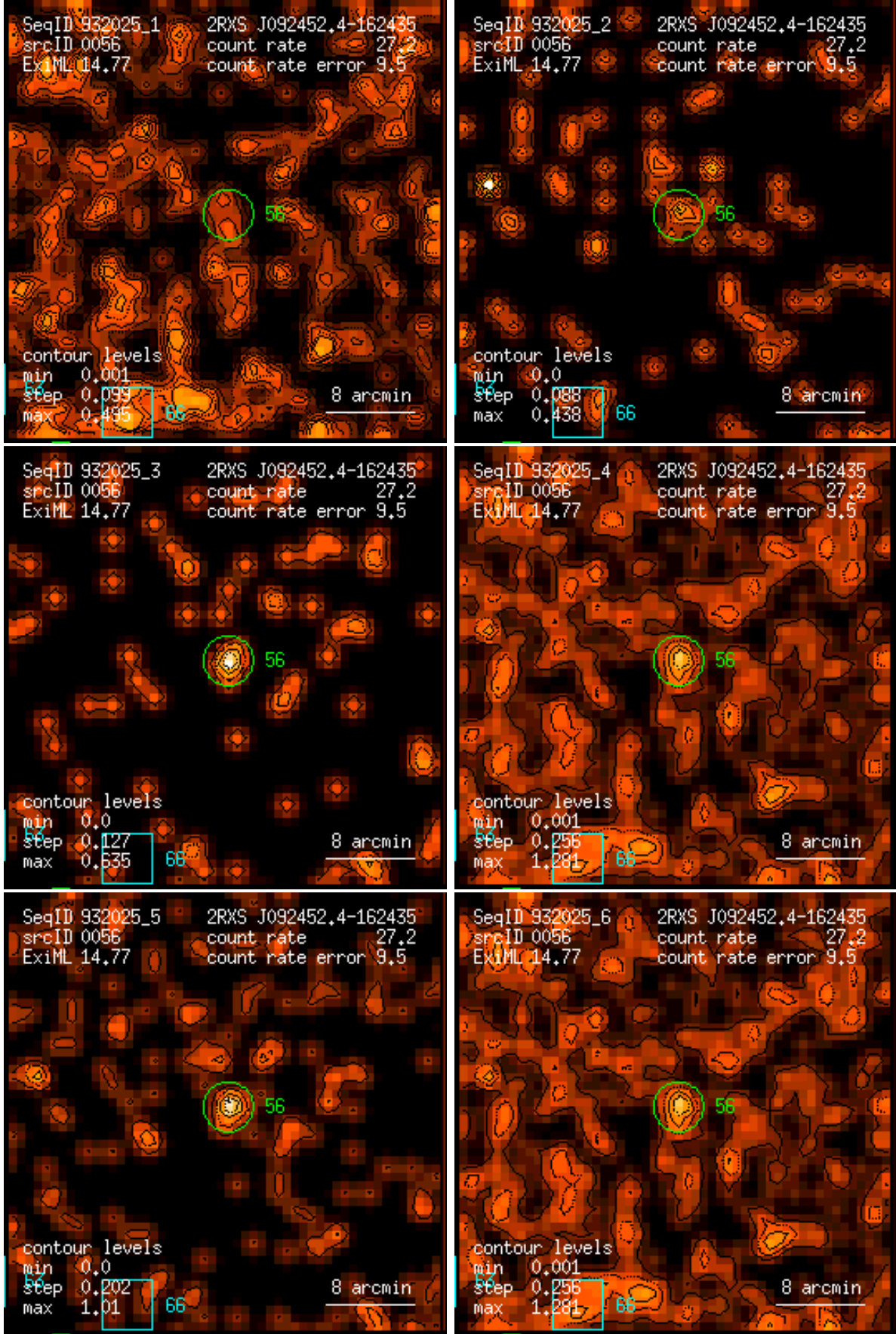
Figure 56: RASS 932025: detection 0056: band rate images, Gaussian filter: (1) PSPC channels 11 – 41, (2) 52 – 90, (3) 91 – 201, (4) 11 – 235, (5) 52 – 201, (6) 11 – 201. Broad band rates in counts/ks. Band rate contour levels in counts/ks/arcmin 2 .
