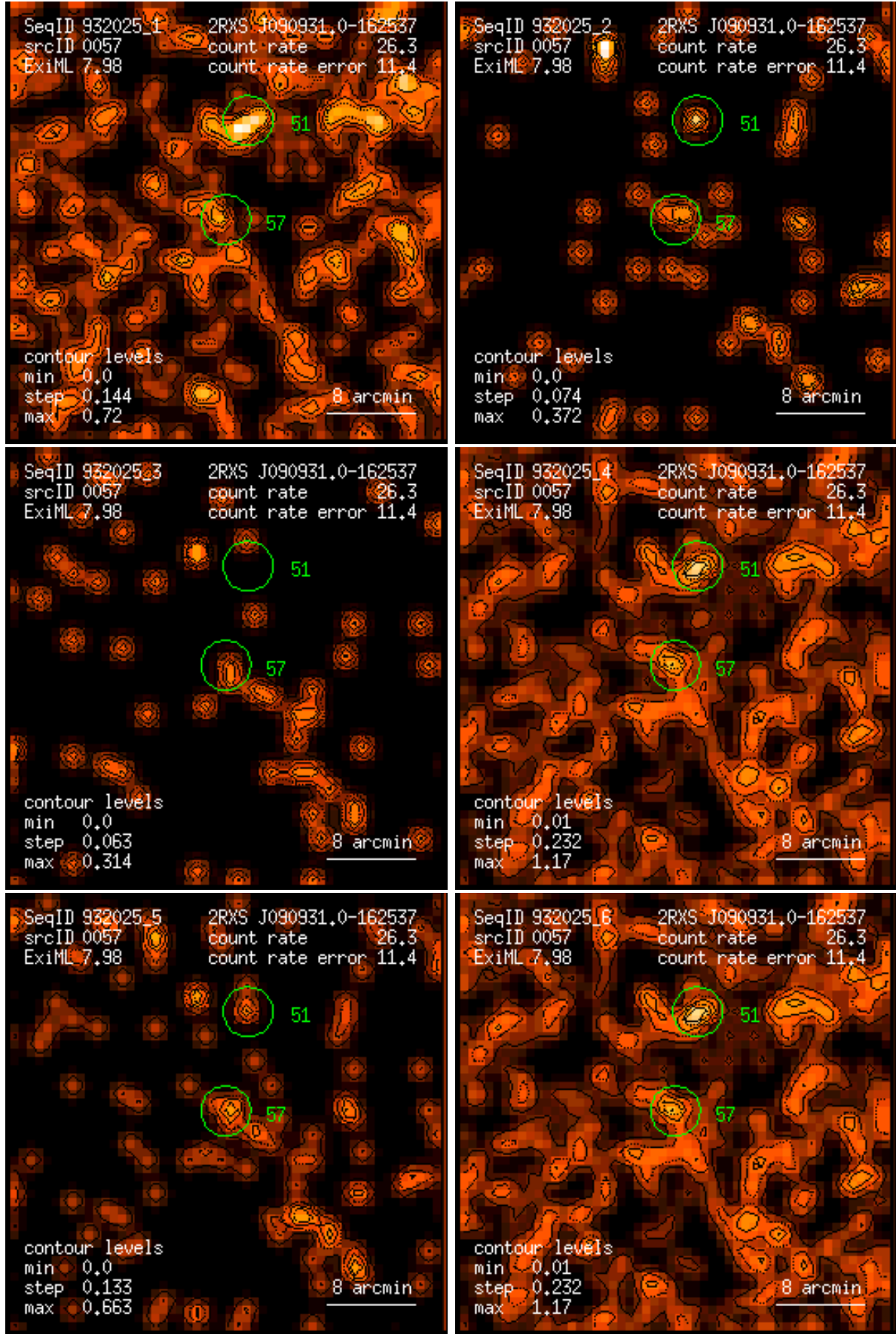
Figure 57: RASS 932025: detection 0057: band rate images, Gaussian filter: (1) PSPC channels 11 – 41, (2) 52 – 90, (3) 91 – 201, (4) 11 – 235, (5) 52 – 201, (6) 11 – 201. Broad band rates in counts/ks. Band rate contour levels in counts/ks/arcmin 2 .
