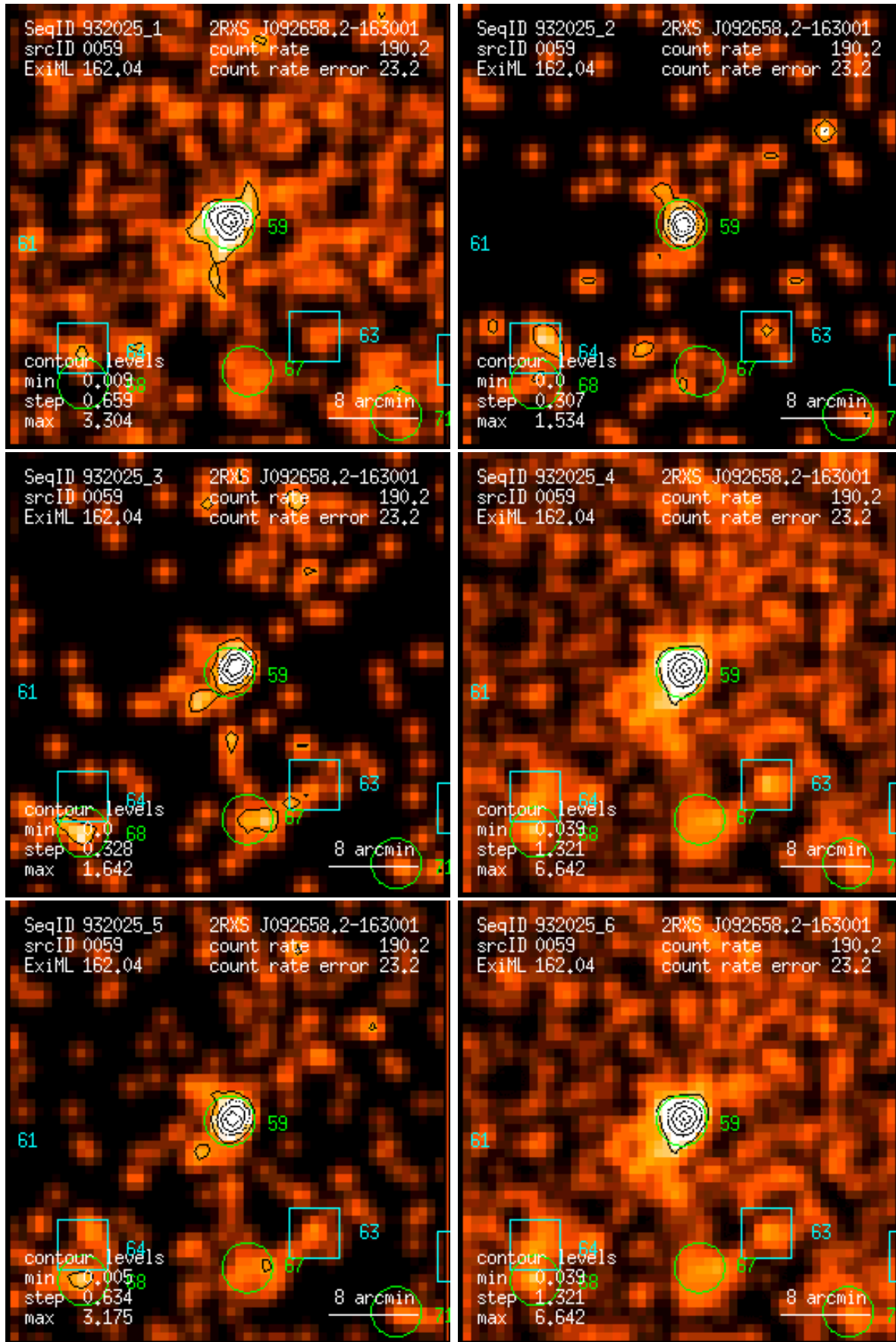
Figure 59: RASS 932025: detection 0059: band rate images, Gaussian filter: (1) PSPC channels 11 – 41, (2) 52 – 90, (3) 91 – 201, (4) 11 – 235, (5) 52 – 201, (6) 11 – 201. Broad band rates in counts/ks. Band rate contour levels in counts/ks/arcmin 2 .
