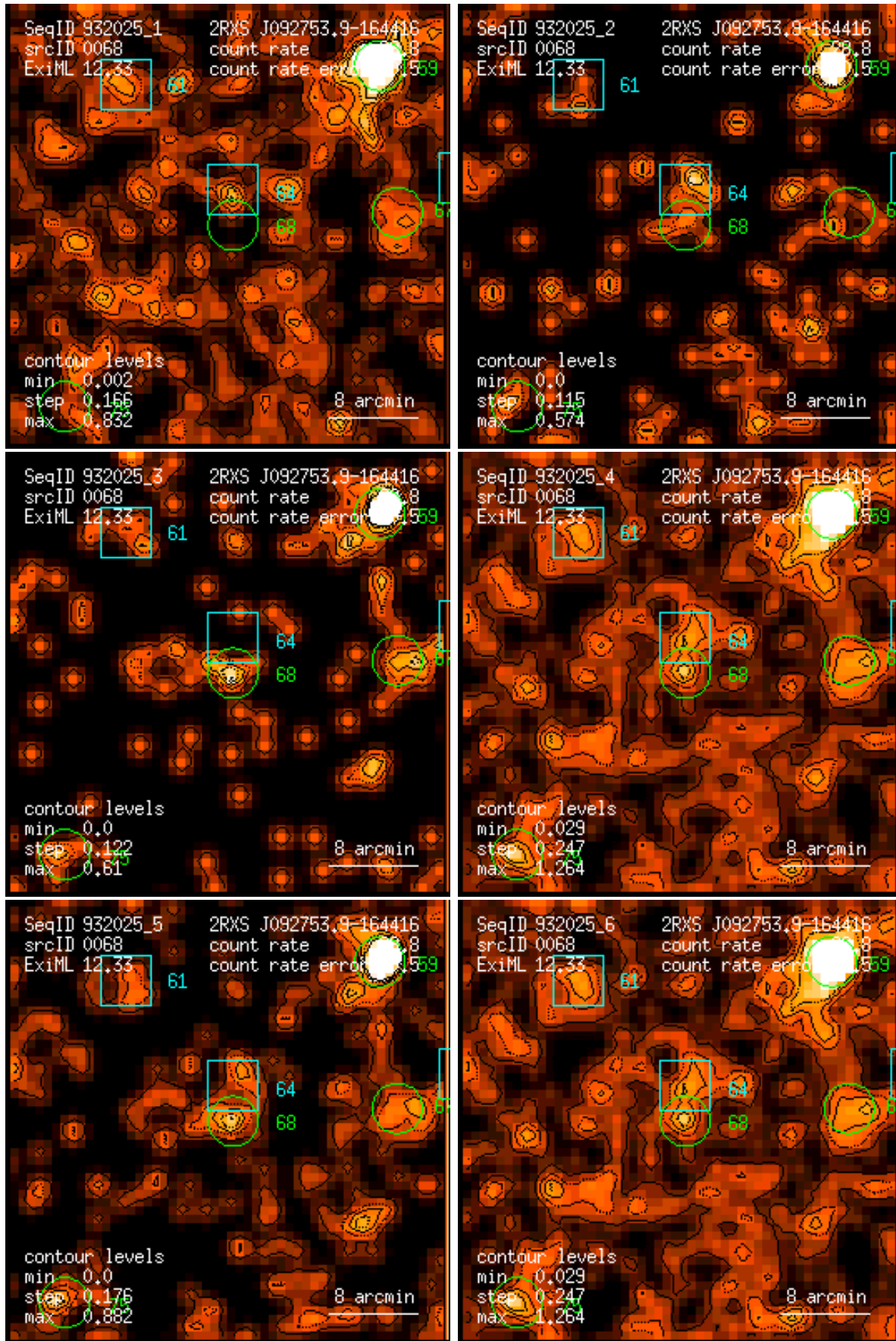
Figure 68: RASS 932025: detection 0068: band rate images, Gaussian filter: (1) PSPC channels 11 – 41, (2) 52 – 90, (3) 91 – 201, (4) 11 – 235, (5) 52 – 201, (6) 11 – 201. Broad band rates in counts/ks. Band rate contour levels in counts/ks/arcmin 2 .
