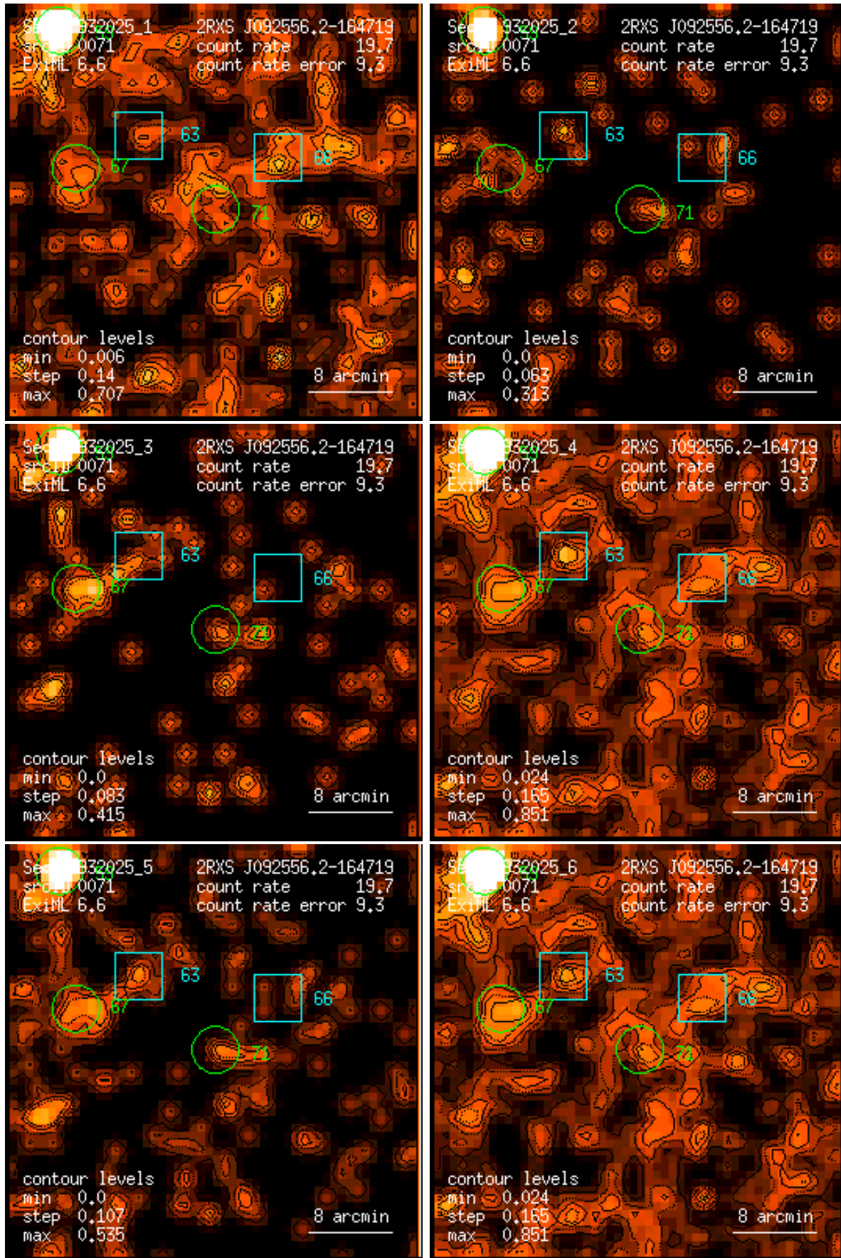
Figure 71: RASS 932025: detection 0071: band rate images, Gaussian filter: (1) PSPC channels 11 – 41, (2) 52 – 90, (3) 91 – 201, (4) 11 – 235, (5) 52 – 201, (6) 11 – 201. Broad band rates in counts/ks. Band rate contour levels in counts/ks/arcmin 2 .
