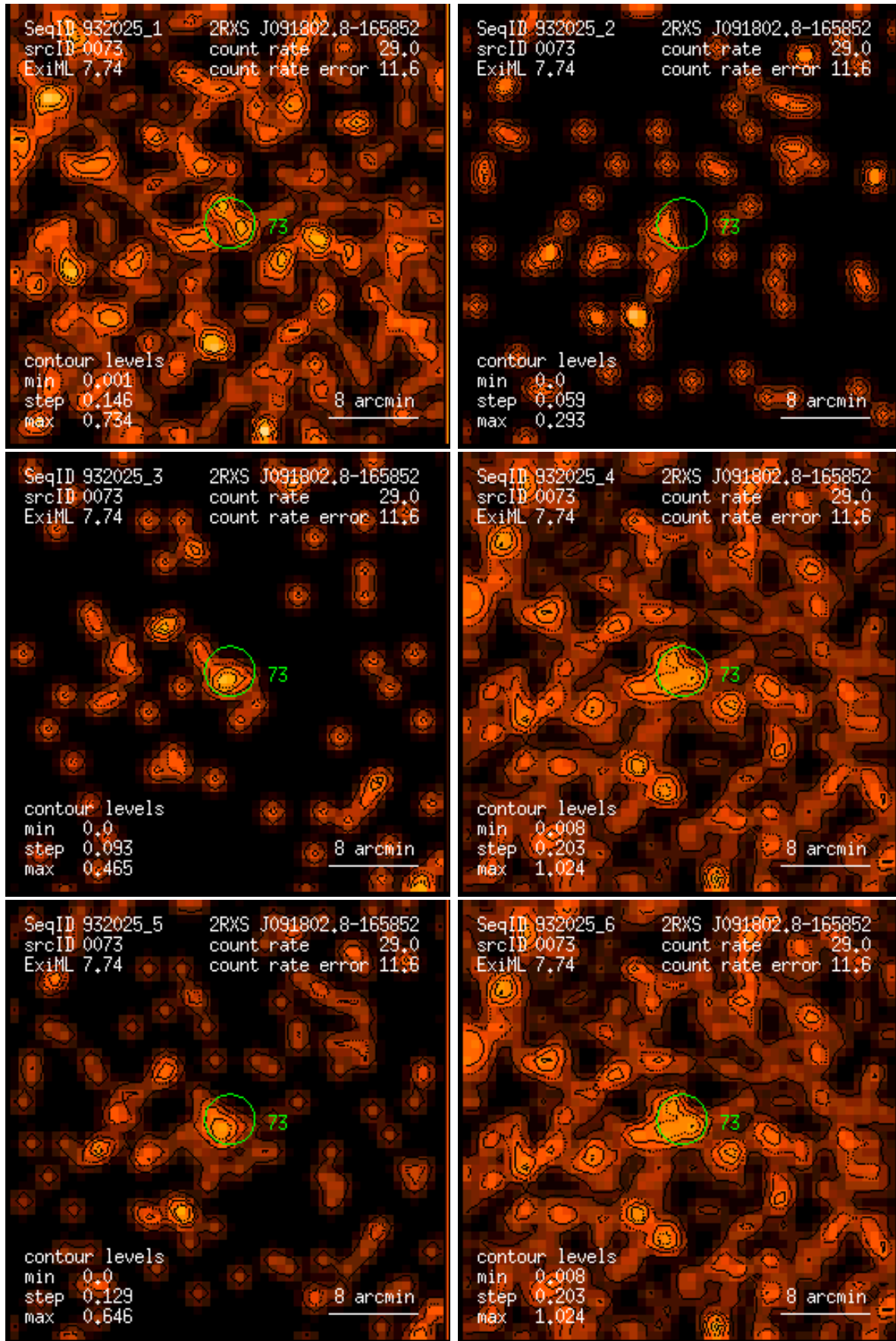
Figure 73: RASS 932025: detection 0073: band rate images, Gaussian filter: (1) PSPC channels 11 – 41, (2) 52 – 90, (3) 91 – 201, (4) 11 – 235, (5) 52 – 201, (6) 11 – 201. Broad band rates in counts/ks. Band rate contour levels in counts/ks/arcmin 2 .
