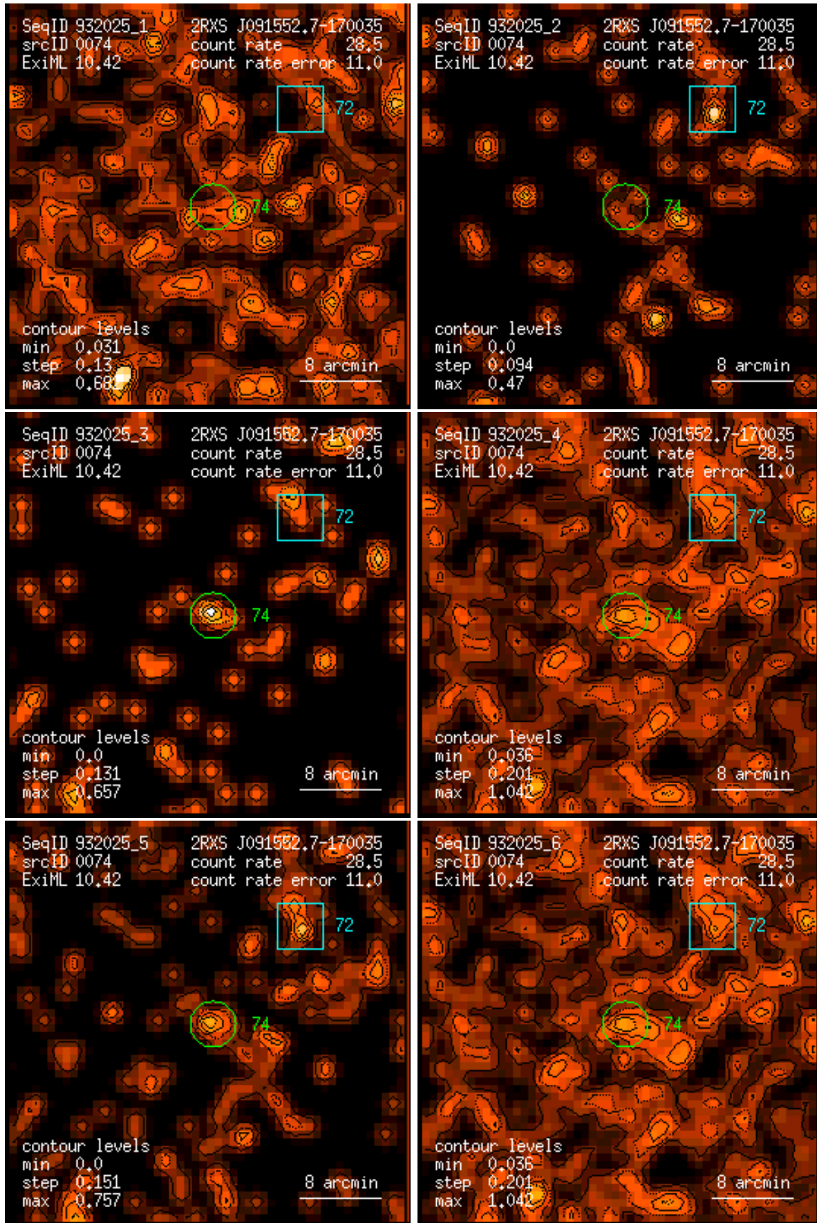
Figure 74: RASS 932025: detection 0074: band rate images, Gaussian filter: (1) PSPC channels 11 – 41, (2) 52 – 90, (3) 91 – 201, (4) 11 – 235, (5) 52 – 201, (6) 11 – 201. Broad band rates in counts/ks. Band rate contour levels in counts/ks/arcmin 2 .
