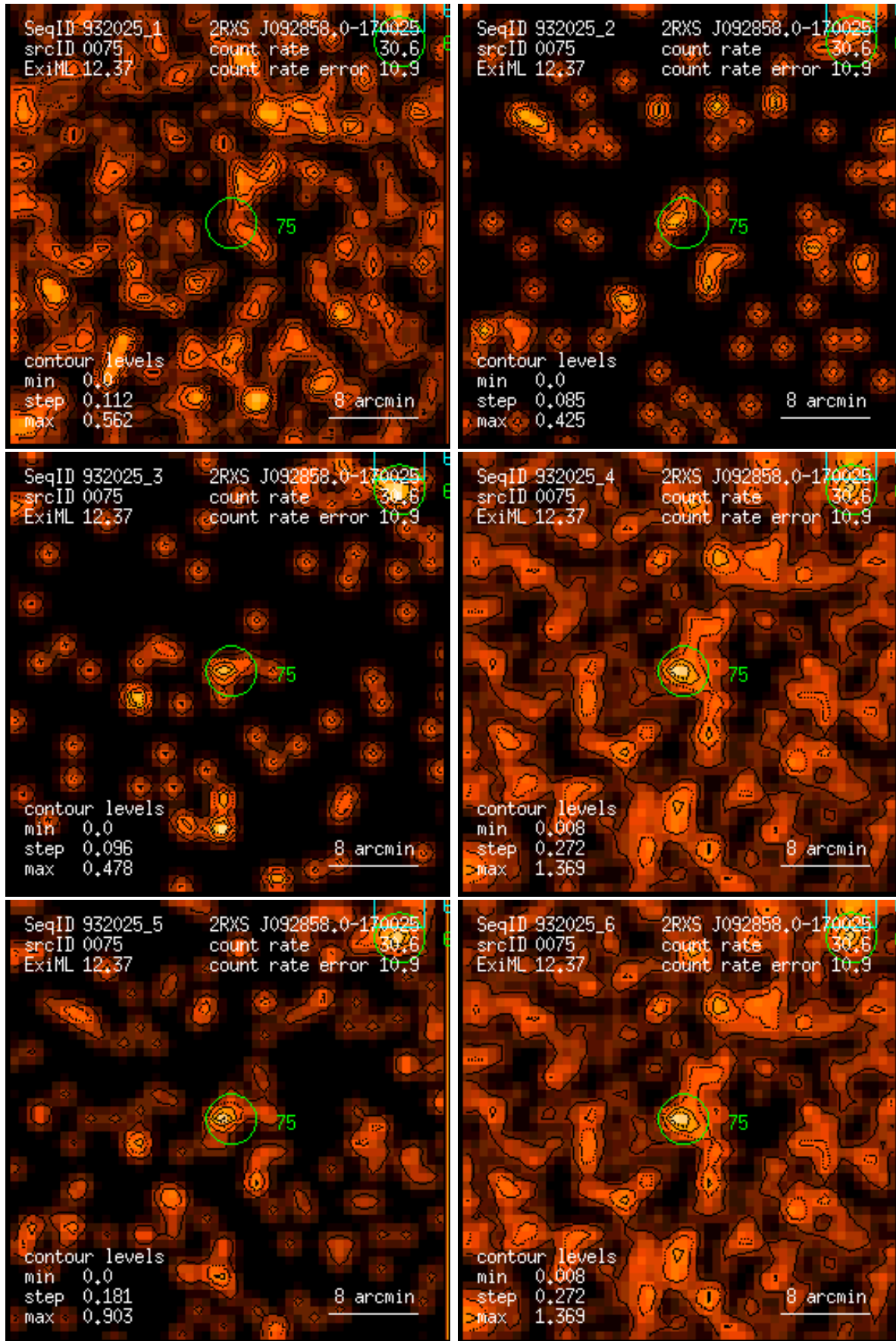
Figure 75: RASS 932025: detection 0075: band rate images, Gaussian filter: (1) PSPC channels 11 – 41, (2) 52 – 90, (3) 91 – 201, (4) 11 – 235, (5) 52 – 201, (6) 11 – 201. Broad band rates in counts/ks. Band rate contour levels in counts/ks/arcmin 2 .
