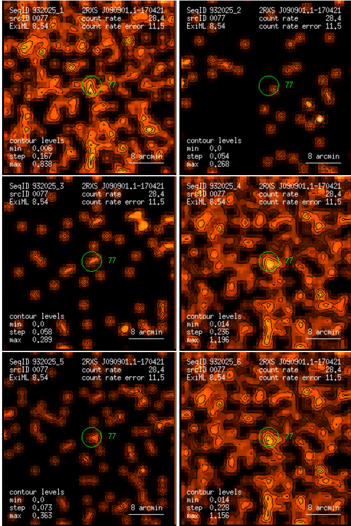
Figure 77: RASS 932025: detection 0077: band rate images, Gaussian filter: (1) PSPC channels 11 – 41, (2) 52 – 90, (3) 91 – 201, (4) 11 – 235, (5) 52 – 201, (6) 11 – 201. Broad band rates in counts/ks. Band rate contour levels in counts/ks/arcmin 2 .
