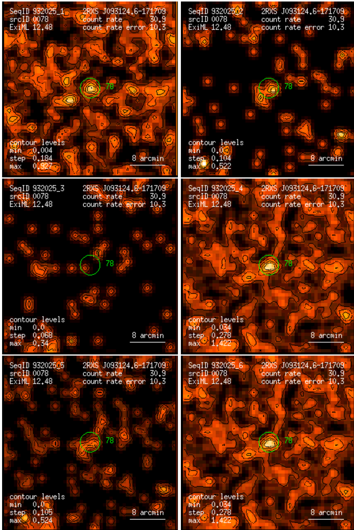
Figure 78: RASS 932025: detection 0078: band rate images, Gaussian filter: (1) PSPC channels 11 – 41, (2) 52 – 90, (3) 91 – 201, (4) 11 – 235, (5) 52 – 201, (6) 11 – 201. Broad band rates in counts/ks. Band rate contour levels in counts/ks/arcmin 2 .
