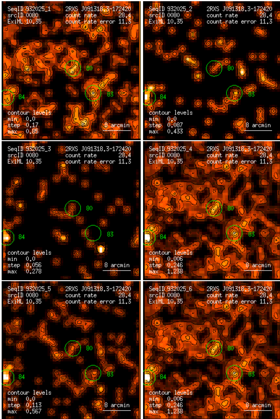
Figure 80: RASS 932025: detection 0080: band rate images, Gaussian filter: (1) PSPC channels 11 – 41, (2) 52 – 90, (3) 91 – 201, (4) 11 – 235, (5) 52 – 201, (6) 11 – 201. Broad band rates in counts/ks. Band rate contour levels in counts/ks/arcmin 2 .
