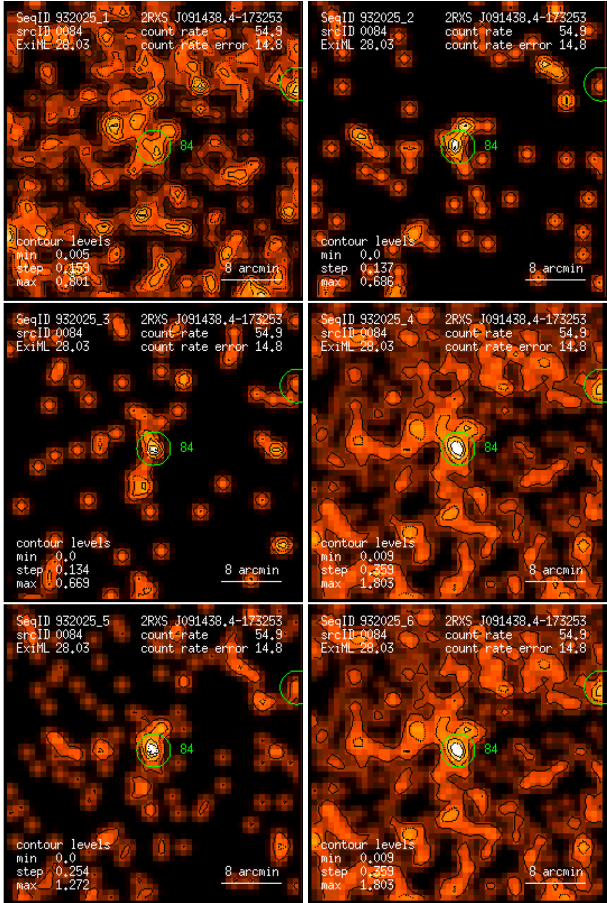
Figure 84: RASS 932025: detection 0084: band rate images, Gaussian filter: (1) PSPC channels 11 – 41, (2) 52 – 90, (3) 91 – 201, (4) 11 – 235, (5) 52 – 201, (6) 11 – 201. Broad band rates in counts/ks. Band rate contour levels in counts/ks/arcmin 2 .
