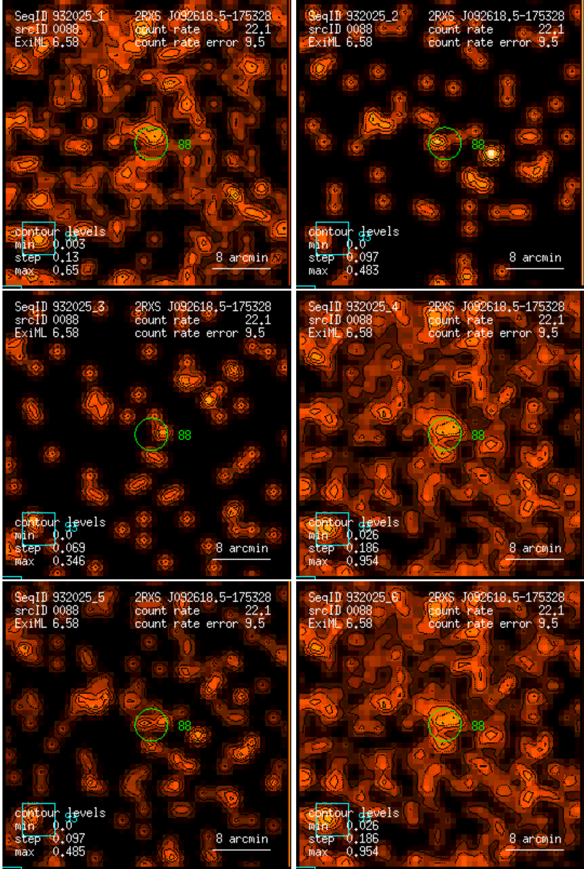
Figure 88: RASS 932025: detection 0088: band rate images, Gaussian filter: (1) PSPC channels 11 – 41, (2) 52 – 90, (3) 91 – 201, (4) 11 – 235, (5) 52 – 201, (6) 11 – 201. Broad band rates in counts/ks. Band rate contour levels in counts/ks/arcmin 2 .
