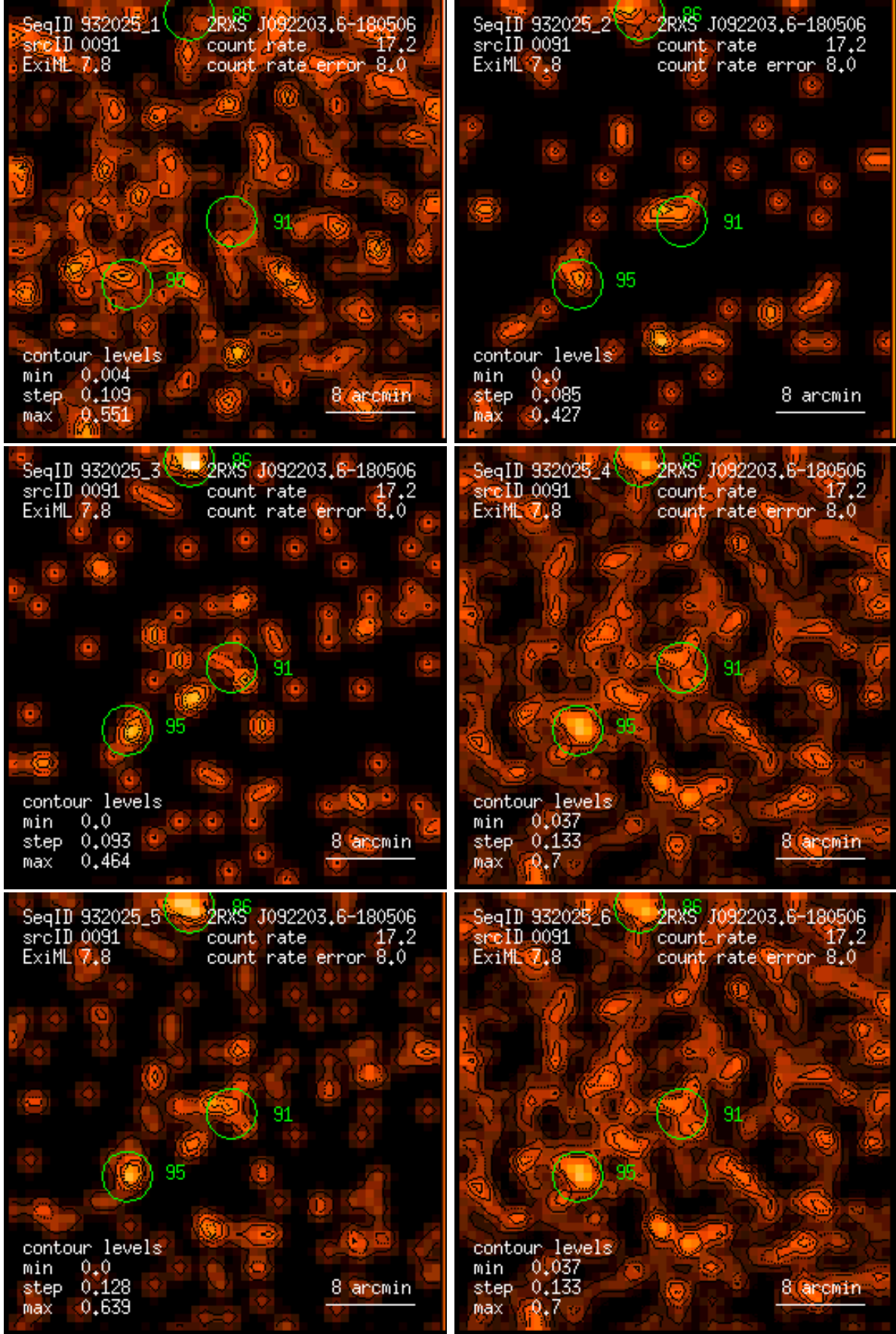
Figure 91: RASS 932025: detection 0091: band rate images, Gaussian filter: (1) PSPC channels 11 – 41, (2) 52 – 90, (3) 91 – 201, (4) 11 – 235, (5) 52 – 201, (6) 11 – 201. Broad band rates in counts/ks. Band rate contour levels in counts/ks/arcmin 2 .
