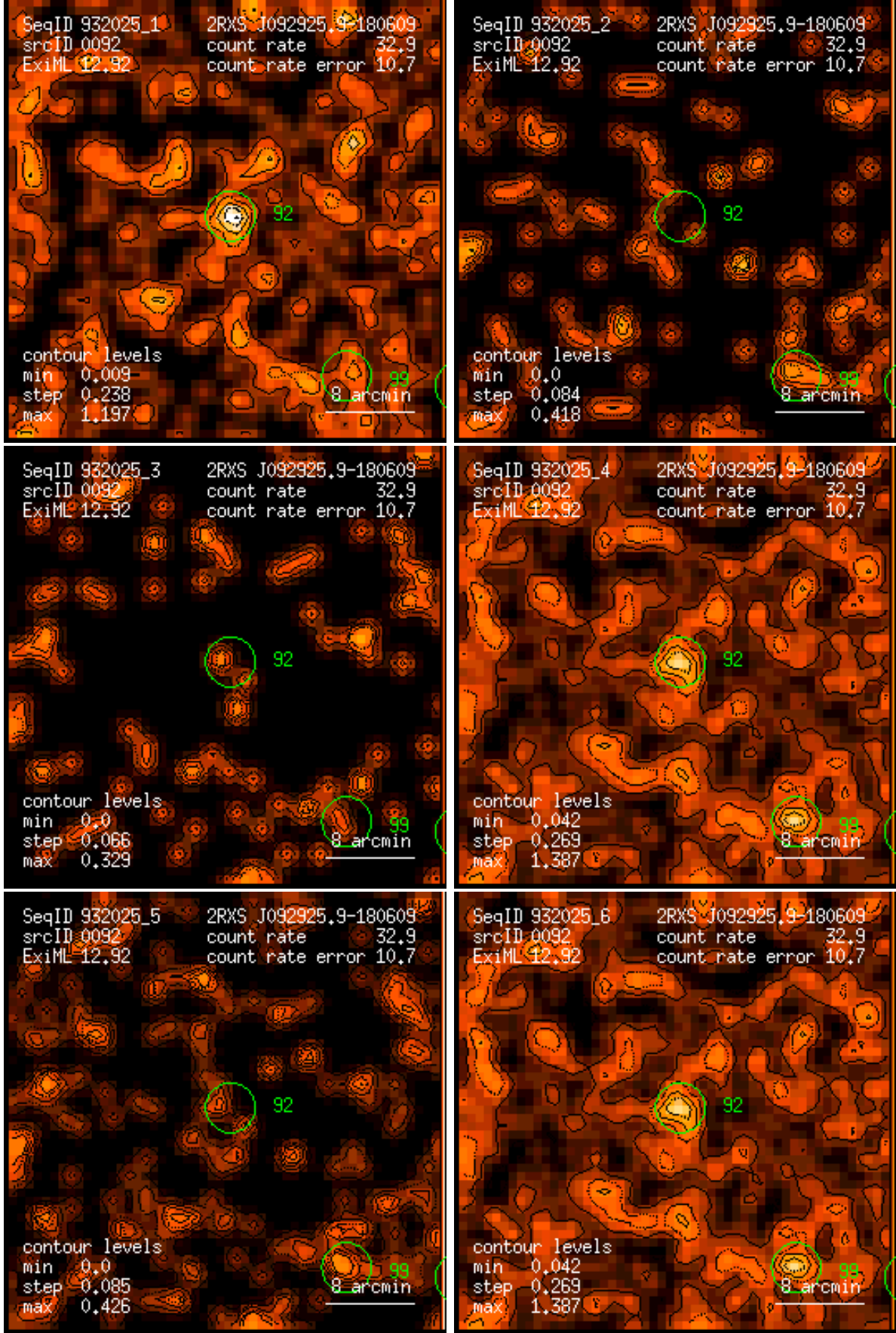
Figure 92: RASS 932025: detection 0092: band rate images, Gaussian filter: (1) PSPC channels 11 – 41, (2) 52 – 90, (3) 91 – 201, (4) 11 – 235, (5) 52 – 201, (6) 11 – 201. Broad band rates in counts/ks. Band rate contour levels in counts/ks/arcmin 2 .
