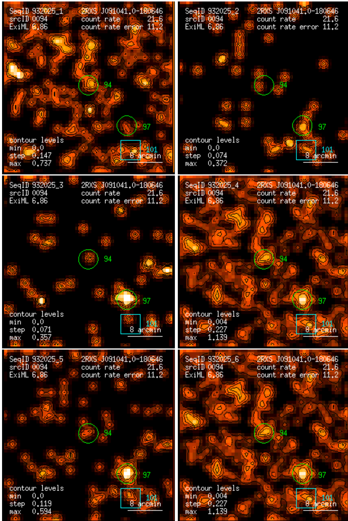
Figure 94: RASS 932025: detection 0094: band rate images, Gaussian filter: (1) PSPC channels 11 – 41, (2) 52 – 90, (3) 91 – 201, (4) 11 – 235, (5) 52 – 201, (6) 11 – 201. Broad band rates in counts/ks. Band rate contour levels in counts/ks/arcmin 2 .
