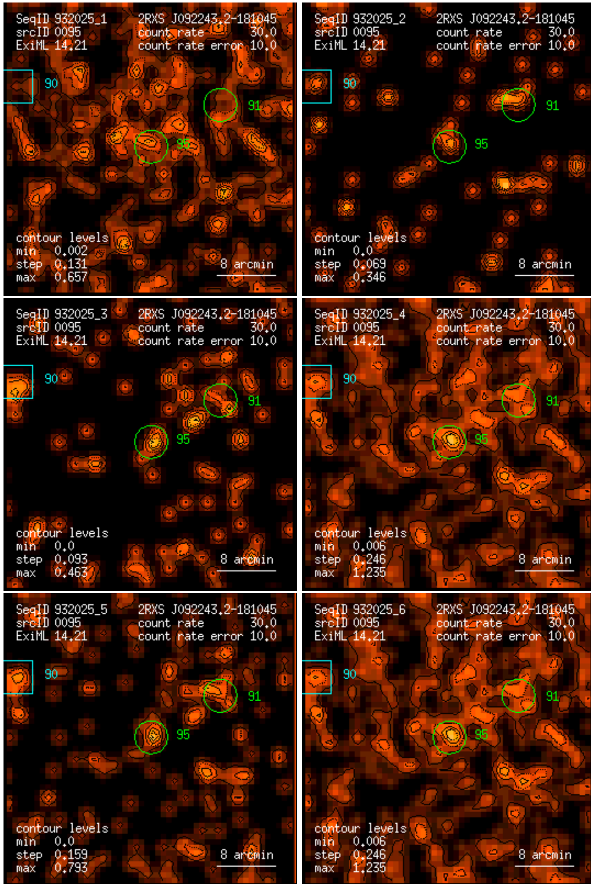
Figure 95: RASS 932025: detection 0095: band rate images, Gaussian filter: (1) PSPC channels 11 – 41, (2) 52 – 90, (3) 91 – 201, (4) 11 – 235, (5) 52 – 201, (6) 11 – 201. Broad band rates in counts/ks. Band rate contour levels in counts/ks/arcmin 2 .
