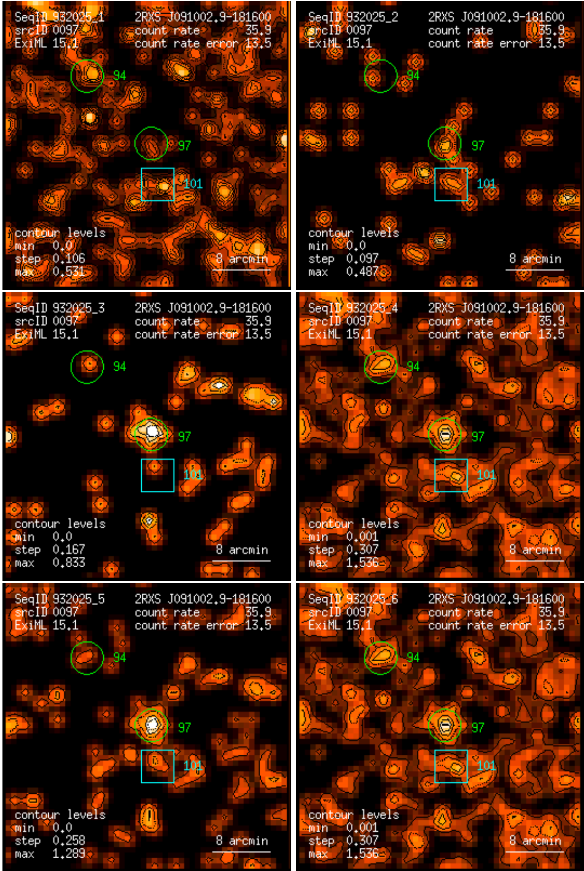
Figure 97: RASS 932025: detection 0097: band rate images, Gaussian filter: (1) PSPC channels 11 – 41, (2) 52 – 90, (3) 91 – 201, (4) 11 – 235, (5) 52 – 201, (6) 11 – 201. Broad band rates in counts/ks. Band rate contour levels in counts/ks/arcmin 2 .
