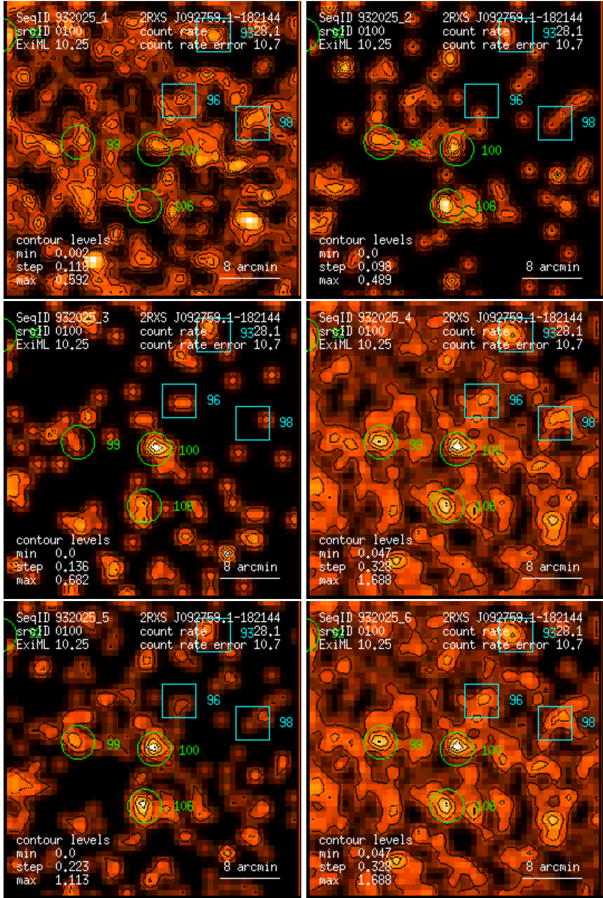
Figure 100: RASS 932025: detection 0100: band rate images, Gaussian filter: (1) PSPC channels 11 – 41, (2) 52 – 90, (3) 91 – 201, (4) 11 – 235, (5) 52 – 201, (6) 11 – 201. Broad band rates in counts/ks. Band rate contour levels in counts/ks/arcmin 2 .
