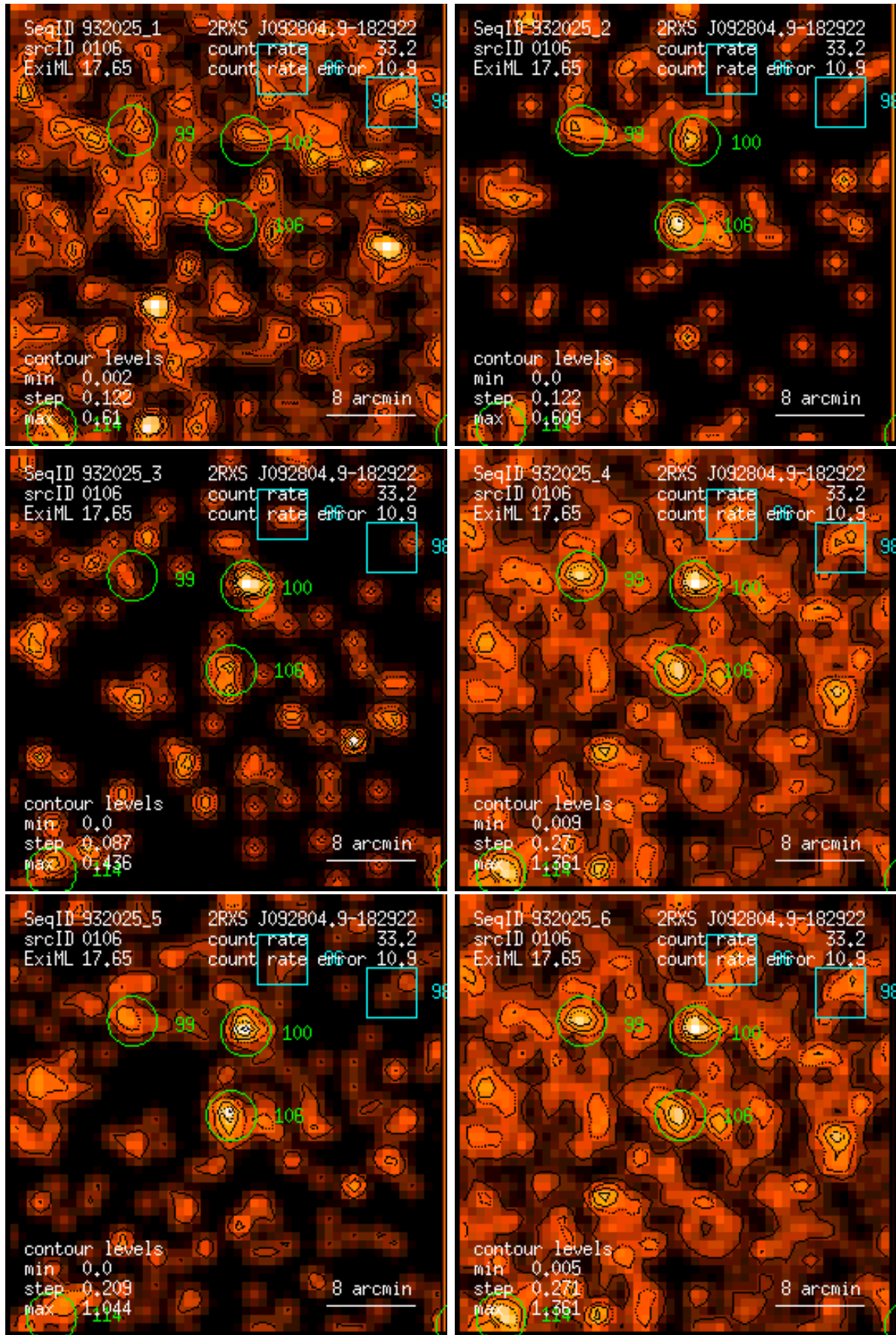
Figure 106: RASS 932025: detection 0106: band rate images, Gaussian filter: (1) PSPC channels 11 – 41, (2) 52 – 90, (3) 91 – 201, (4) 11 – 235, (5) 52 – 201, (6) 11 – 201. Broad band rates in counts/ks. Band rate contour levels in counts/ks/arcmin 2 .
