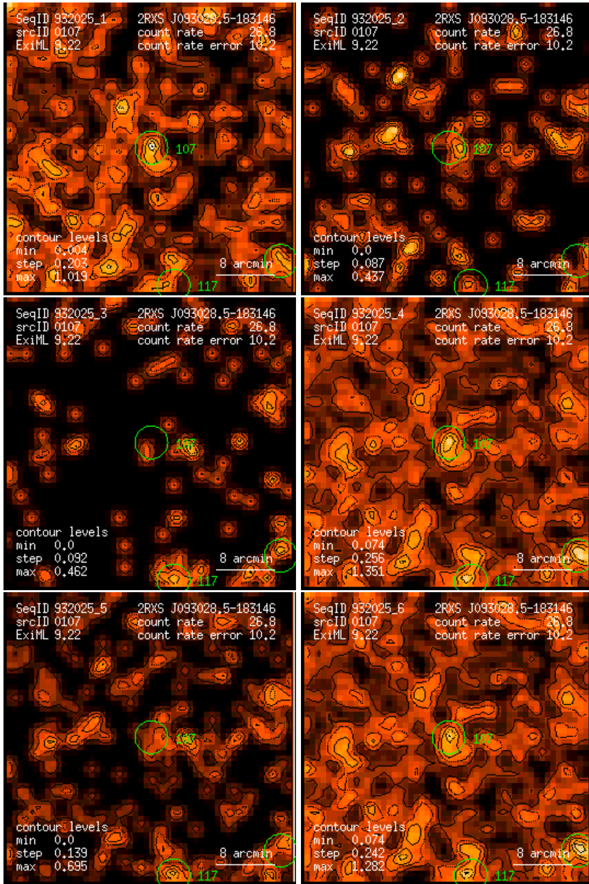
Figure 107: RASS 932025: detection 0107: band rate images, Gaussian filter: (1) PSPC channels 11 – 41, (2) 52 – 90, (3) 91 – 201, (4) 11 – 235, (5) 52 – 201, (6) 11 – 201. Broad band rates in counts/ks. Band rate contour levels in counts/ks/arcmin 2 .
