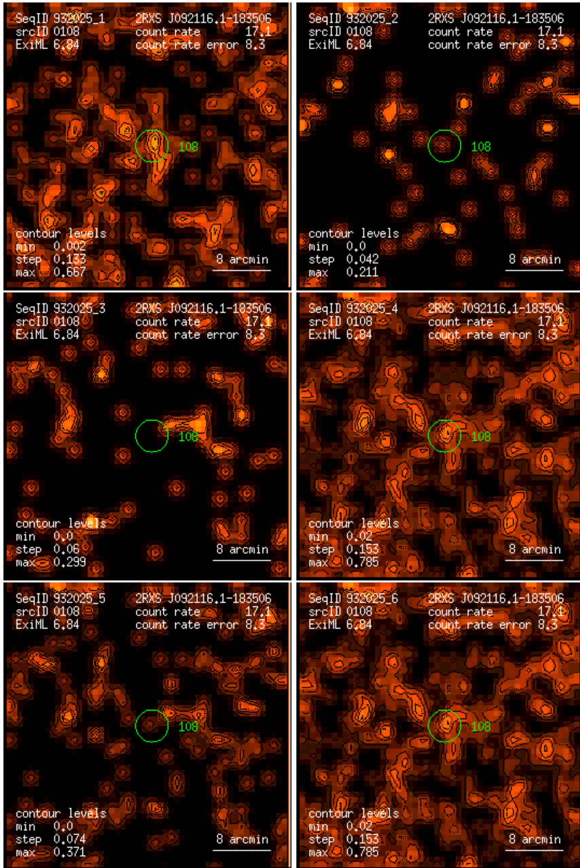
Figure 108: RASS 932025: detection 0108: band rate images, Gaussian filter: (1) PSPC channels 11 – 41, (2) 52 – 90, (3) 91 – 201, (4) 11 – 235, (5) 52 – 201, (6) 11 – 201. Broad band rates in counts/ks. Band rate contour levels in counts/ks/arcmin 2 .
