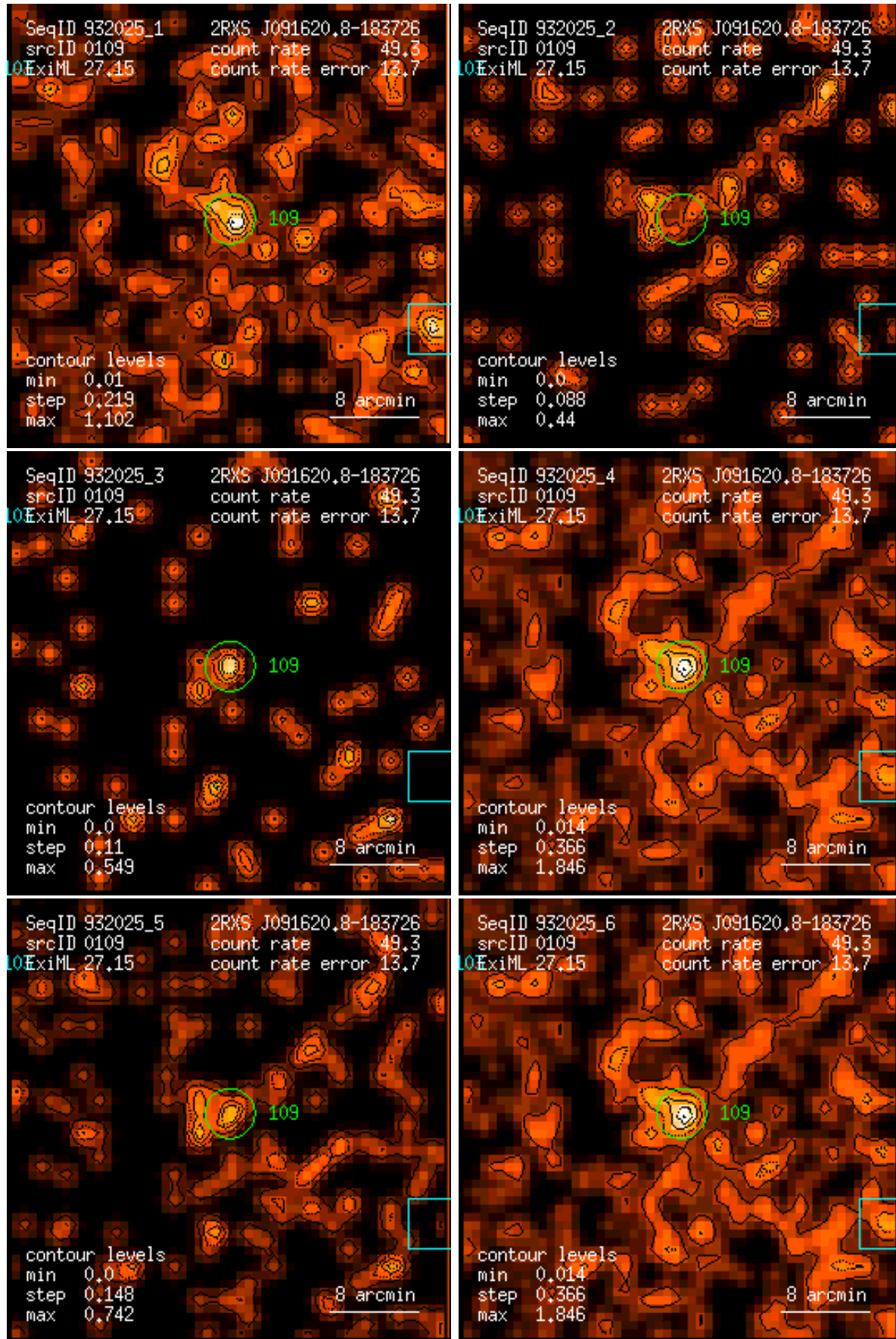
Figure 109: RASS 932025: detection 0109: band rate images, Gaussian filter: (1) PSPC channels 11 – 41, (2) 52 – 90, (3) 91 – 201, (4) 11 – 235, (5) 52 – 201, (6) 11 – 201. Broad band rates in counts/ks. Band rate contour levels in counts/ks/arcmin 2 .
