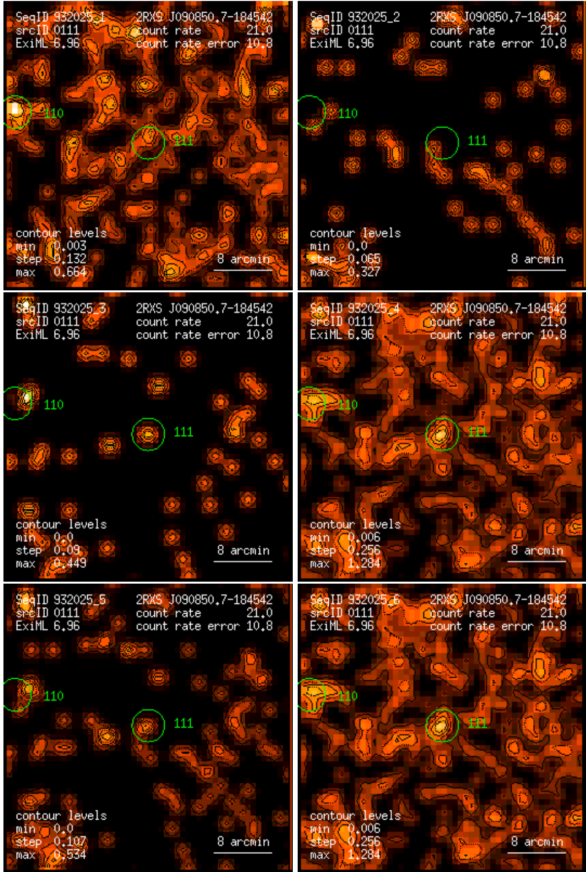
Figure 111: RASS 932025: detection 0111: band rate images, Gaussian filter: (1) PSPC channels 11 – 41, (2) 52 – 90, (3) 91 – 201, (4) 11 – 235, (5) 52 – 201, (6) 11 – 201. Broad band rates in counts/ks. Band rate contour levels in counts/ks/arcmin 2 .
