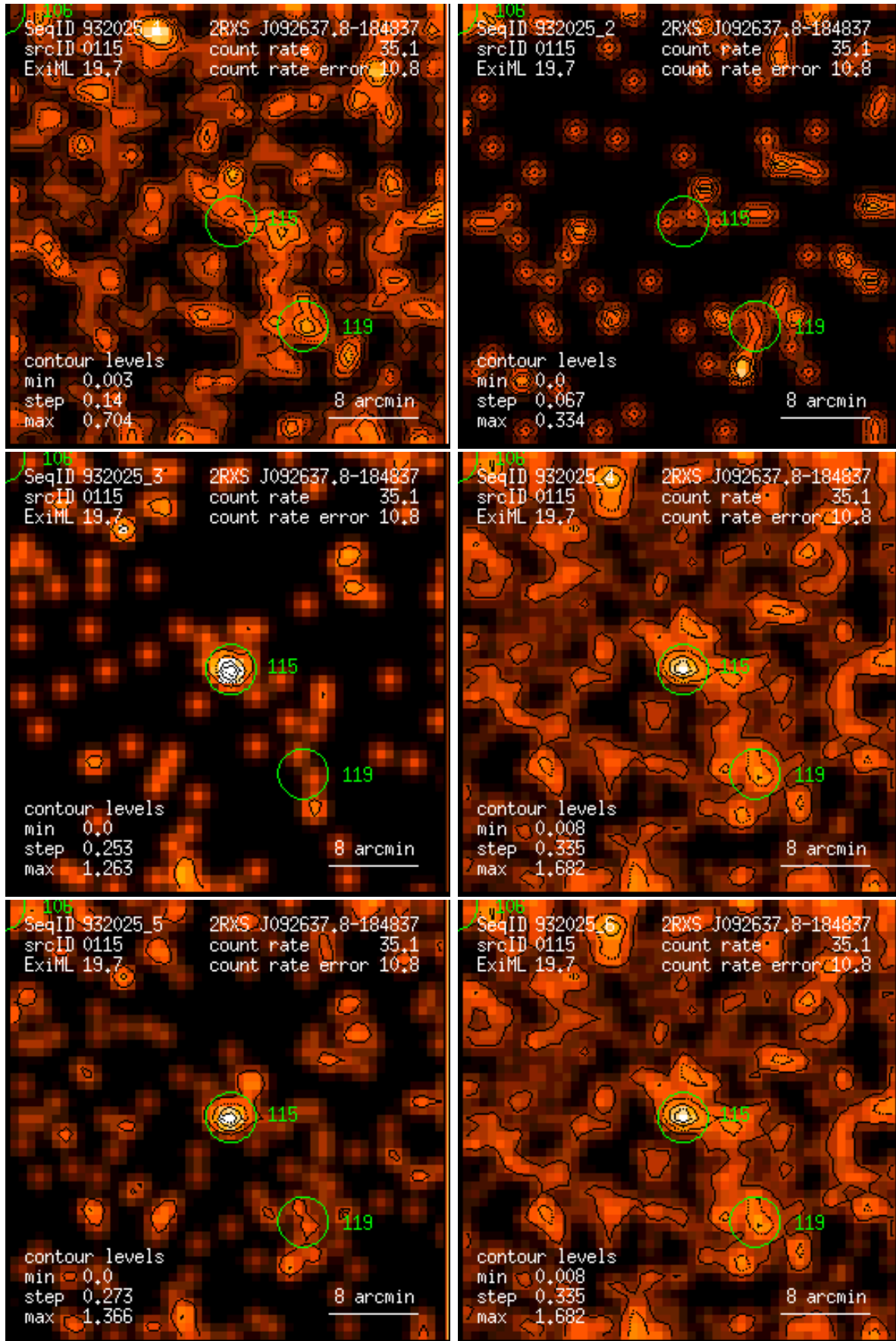
Figure 115: RASS 932025: detection 0115: band rate images, Gaussian filter: (1) PSPC channels 11 – 41, (2) 52 – 90, (3) 91 – 201, (4) 11 – 235, (5) 52 – 201, (6) 11 – 201. Broad band rates in counts/ks. Band rate contour levels in counts/ks/arcmin 2 .
