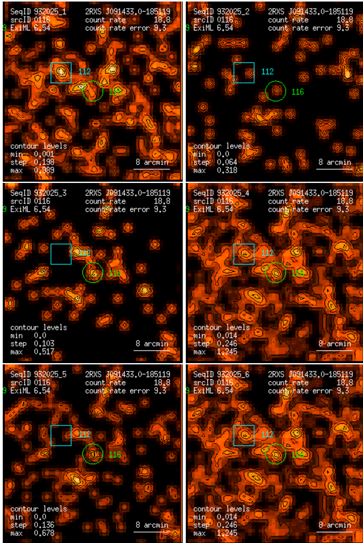
Figure 116: RASS 932025: detection 0116: band rate images, Gaussian filter: (1) PSPC channels 11 – 41, (2) 52 – 90, (3) 91 – 201, (4) 11 – 235, (5) 52 – 201, (6) 11 – 201. Broad band rates in counts/ks. Band rate contour levels in counts/ks/arcmin 2 .
