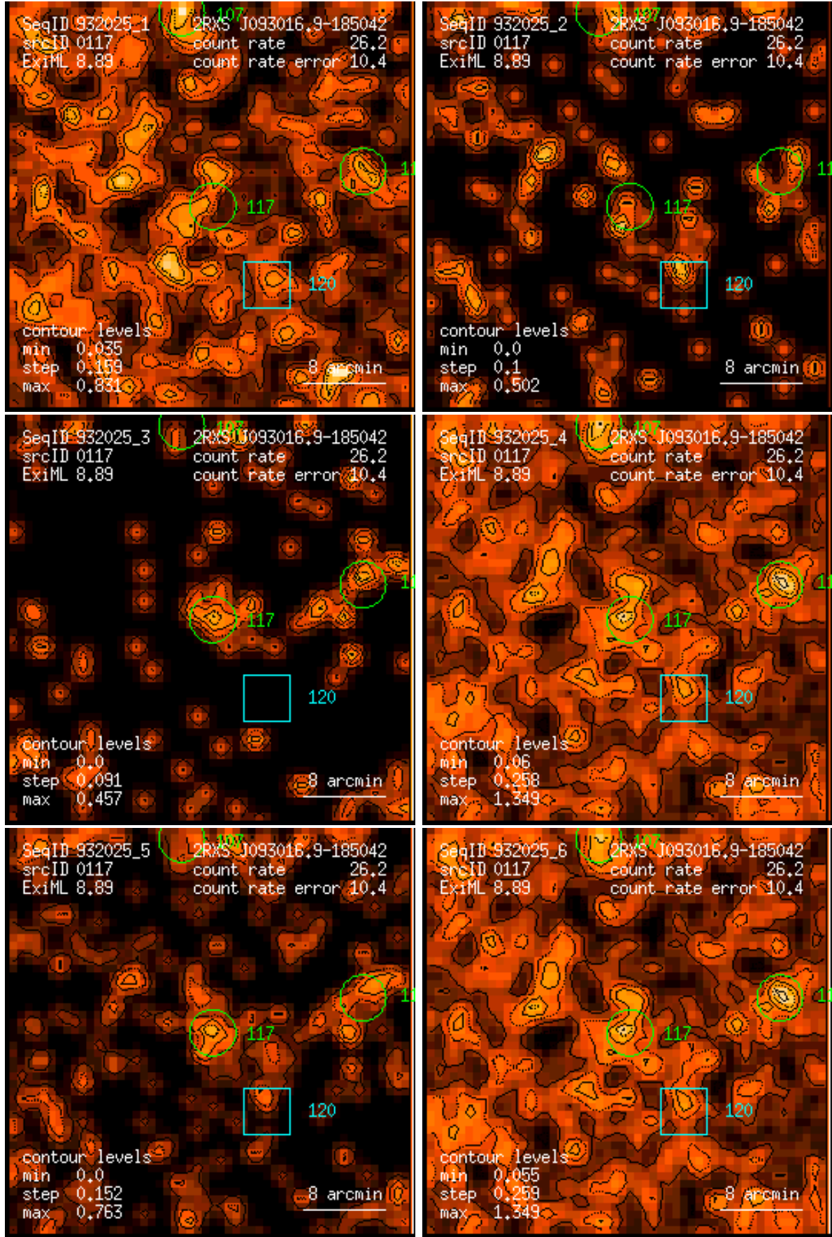
Figure 117: RASS 932025: detection 0117: band rate images, Gaussian filter: (1) PSPC channels 11 – 41, (2) 52 – 90, (3) 91 – 201, (4) 11 – 235, (5) 52 – 201, (6) 11 – 201. Broad band rates in counts/ks. Band rate contour levels in counts/ks/arcmin 2 .
